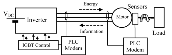
Fig. 3. PLC-based motor feedback loop after [12]. The communication signal shares the feeder cable with the PWM power waveform.
