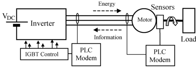
Fig. 4. PLC-based motor feedback loop after [12]. The communication signal shares the feeder cable with the PWM power waveform.
