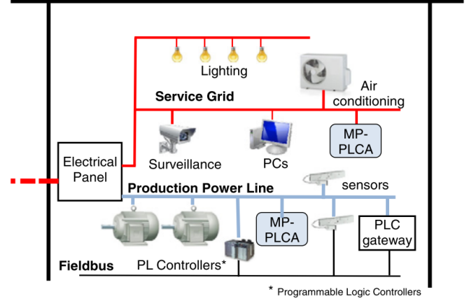
Fig. 3. Example of devices present in the industrial environment
