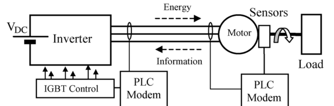
Fig. 3. PLC-based motor feedback loop after [11]. The communication signal shares the feeder cable with the PWM power waveform.
