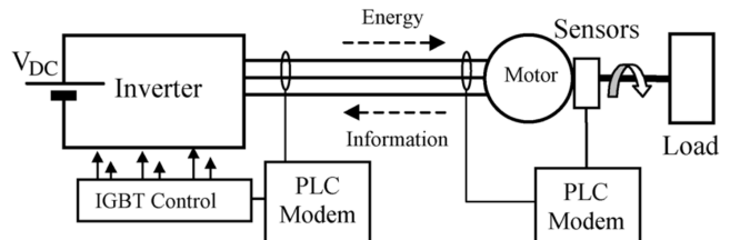
Fig. 3. PLC-based motor feedback loop after [11]. The communication signal shares the feeder cable with the PWM power waveform.
