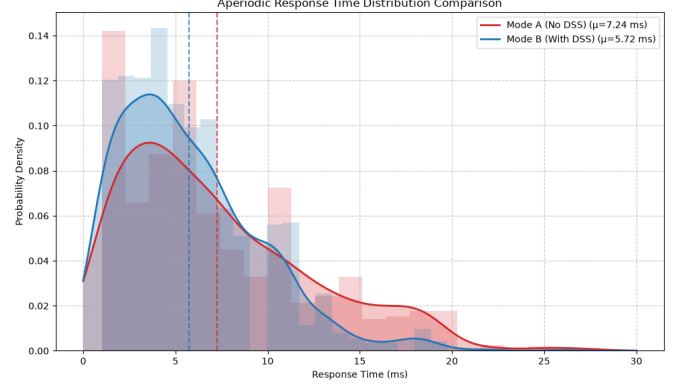
Fig. 5. C_s = 12 , T_s = 25 .
