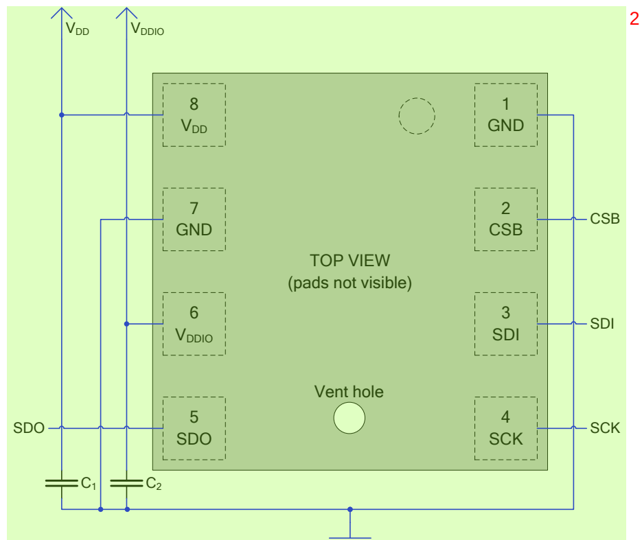
Figure 18: 4-wire SPI connection diagram 3
