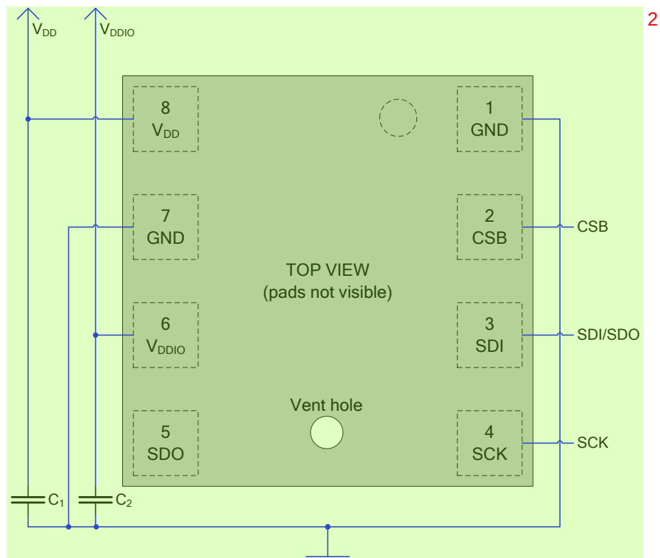
Figure 19: 3-wire SPI connection diagram 3
