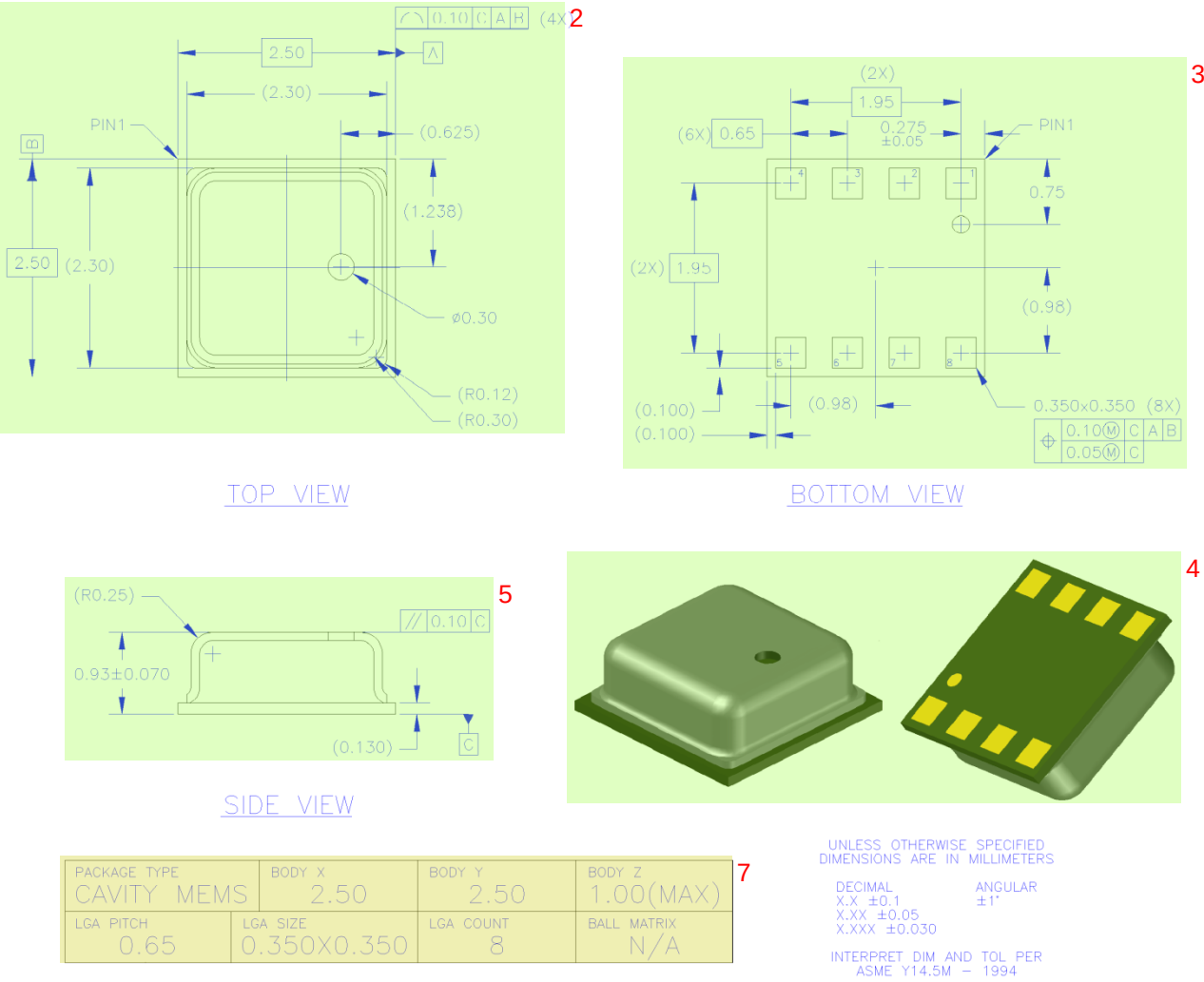
Figure 20: Package dimensions for top, bottom and side view 6
