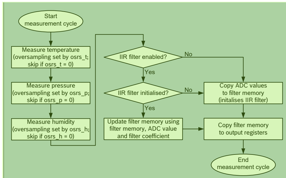
Figure 6: BME280 measurement cycle 4
