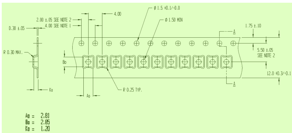
Figure 23: Tape and Reel dimensions 11
