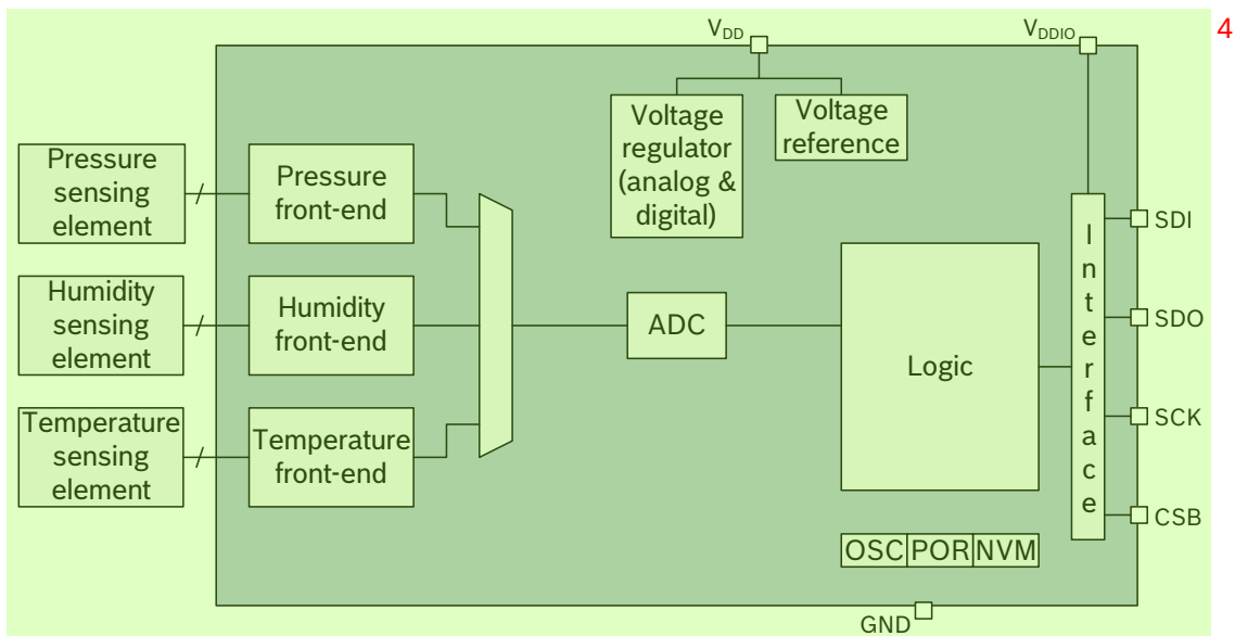
Figure 2: Block diagram of BME280 5
