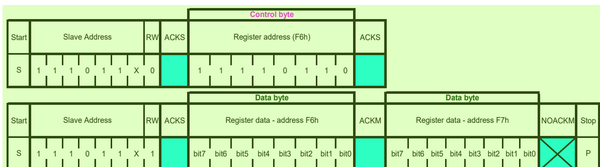
Figure 10: I 2 C multiple byte read
