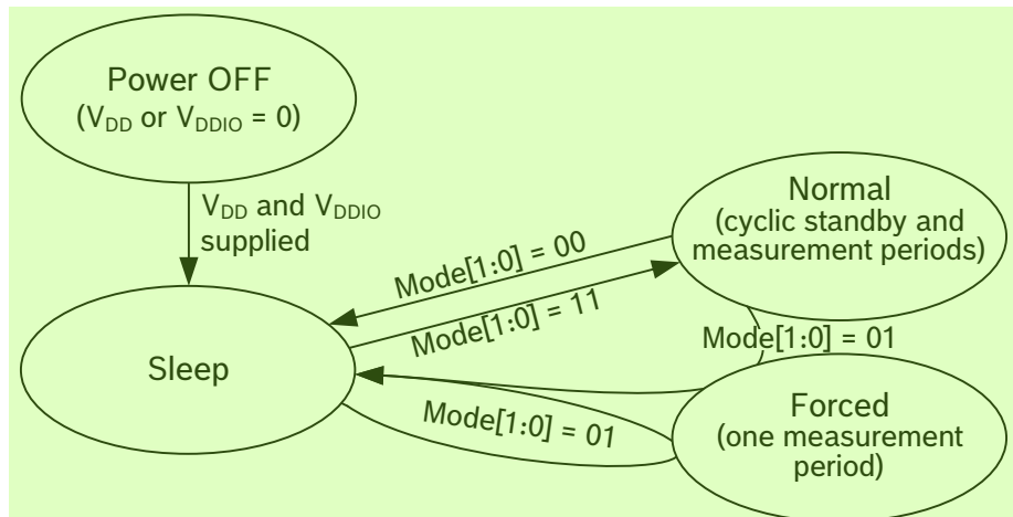
Figure 3: Sensor mode transition diagram 4
