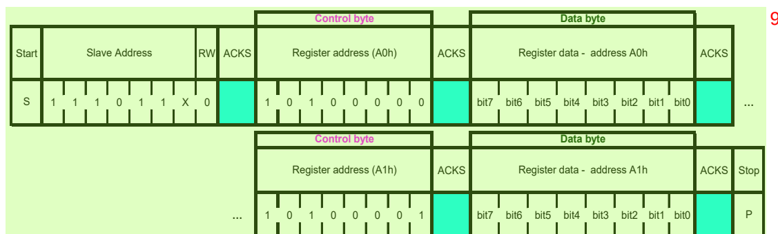
Figure 9: I 2 C multiple byte write (not auto-incremented)
