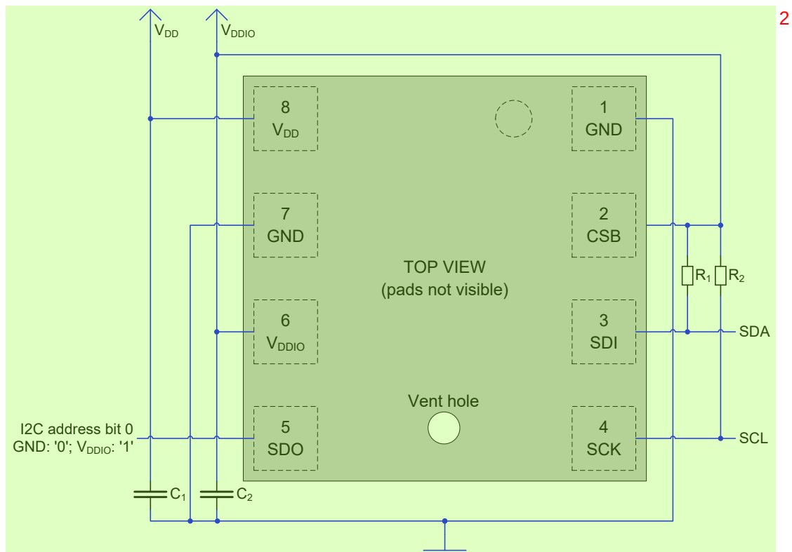
Figure 17: I 2 C connection diagram 3
