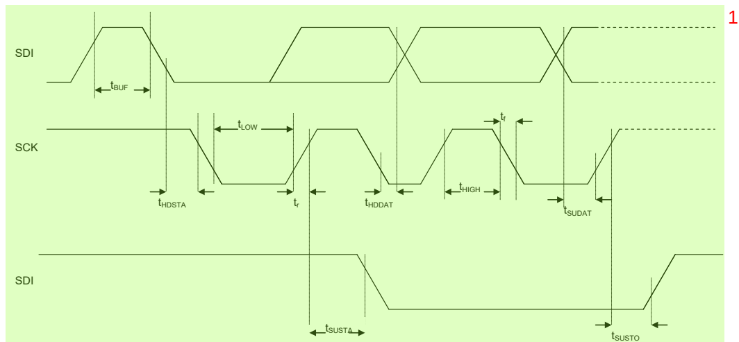
Figure 14: I²C timing diagram 2
