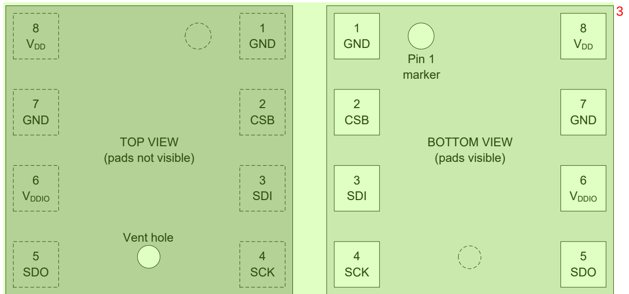
Figure 16: Pin-out top and bottom view 4
