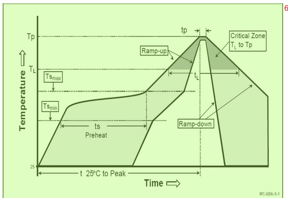
Figure 22: Soldering profile 7
