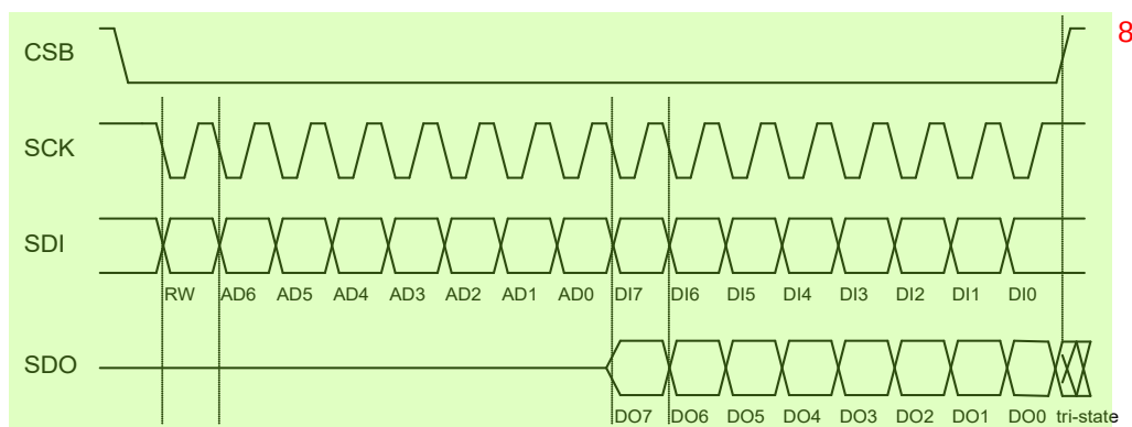
Figure 11: SPI protocol (shown for mode '11' in 4-wire configuration) 8
