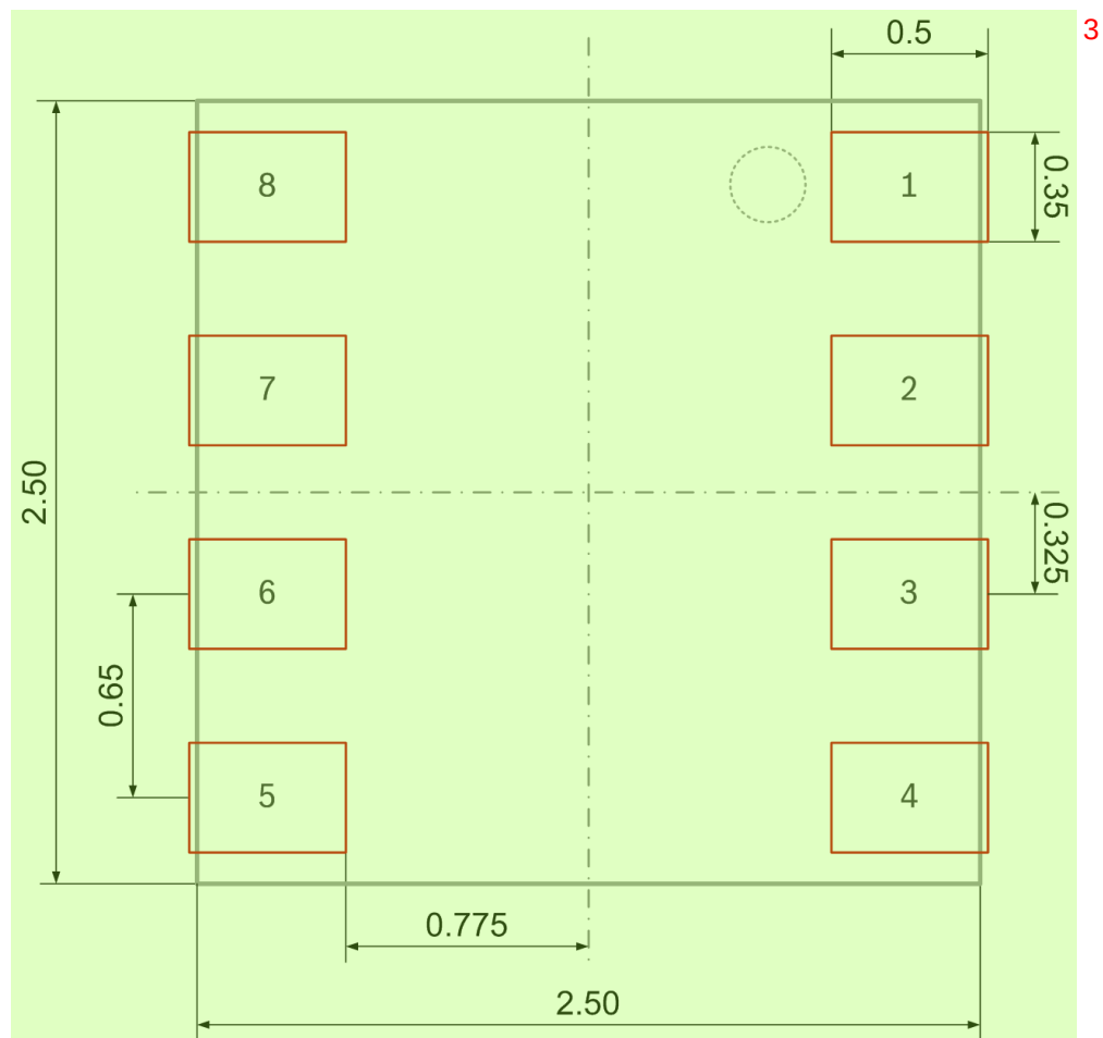
Figure 21: Recommended landing pattern (top view) 4
