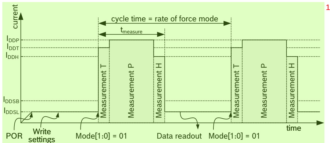
Figure 4: Forced mode timing diagram 2
