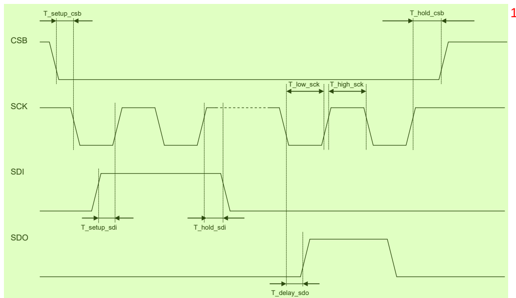
Figure 15: SPI timing diagram 2
