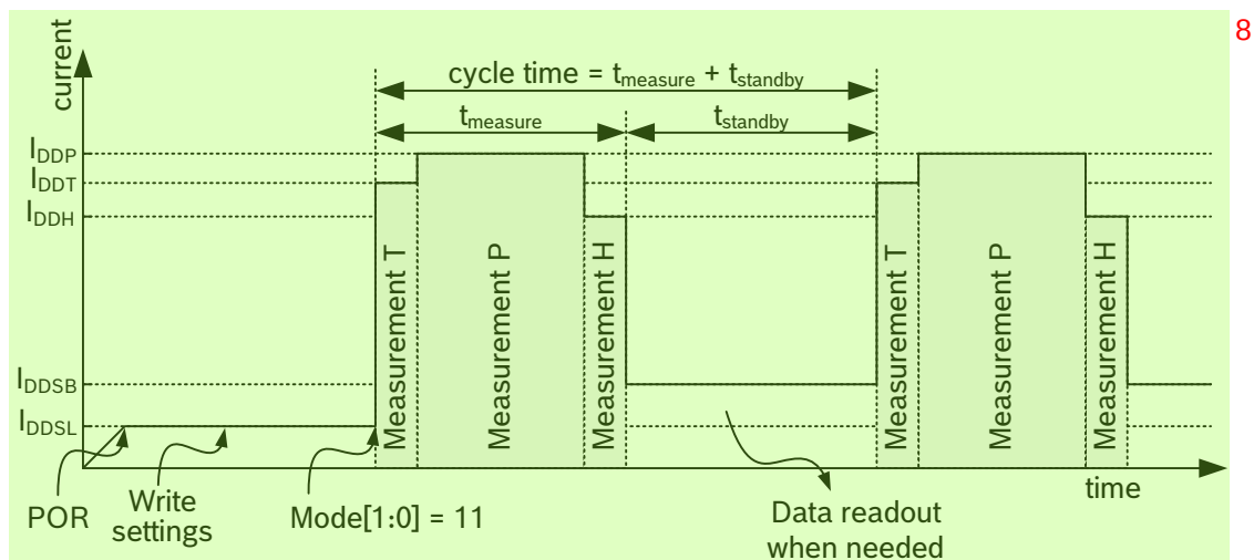
Figure 5: Normal mode timing diagram 9
