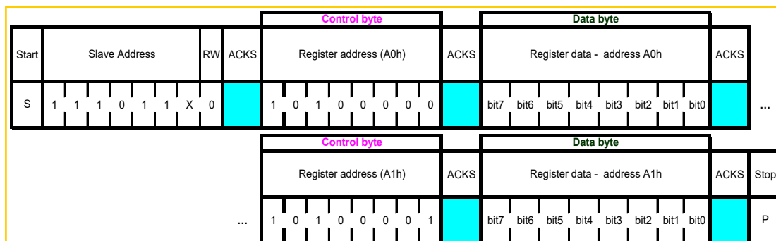
Figure 9: I 2 C multiple byte write (not auto-incremented)
