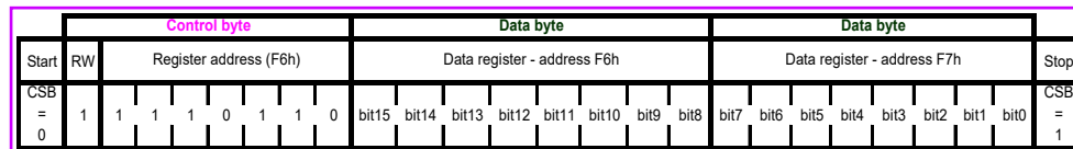
Figure 13: SPI multiple byte read
