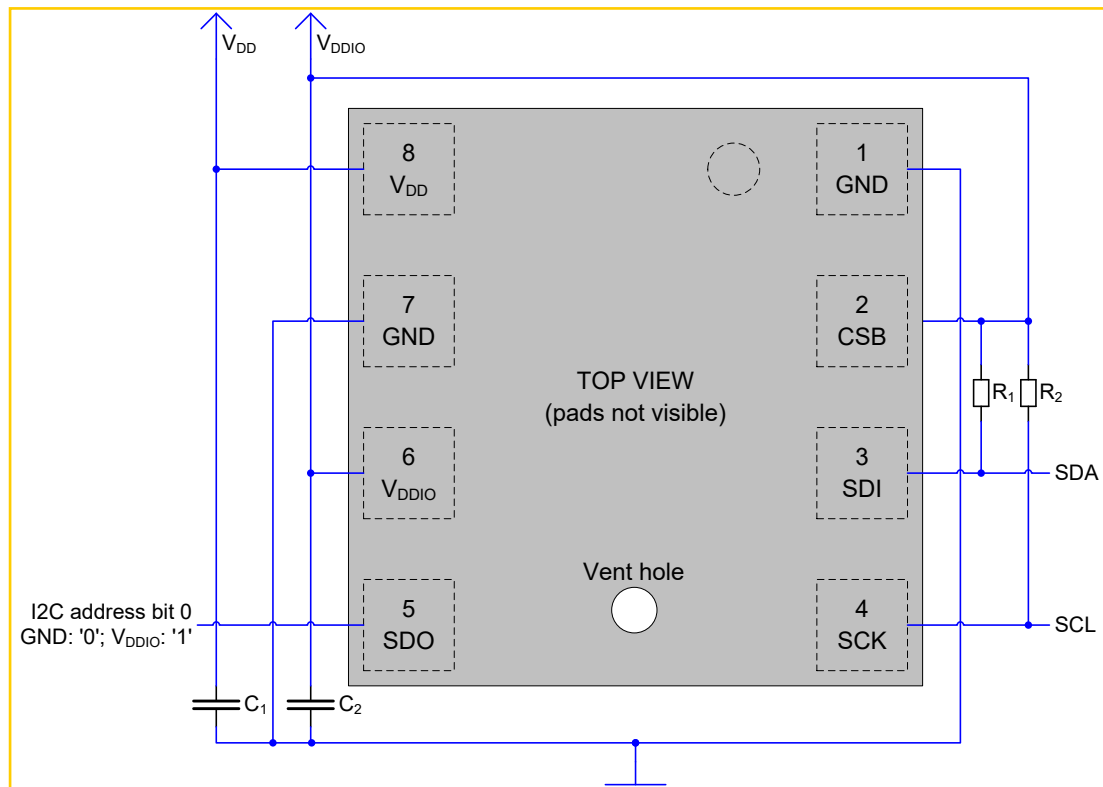
Figure 17: I 2 C connection diagram
