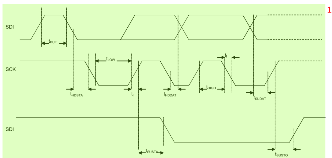
Figure 12: I²C timing diagram 2
