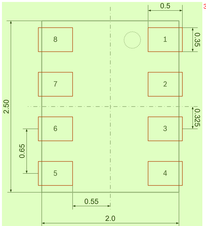
Figure 19: Recommended landing pattern (top view); dimensions are in mm 4
