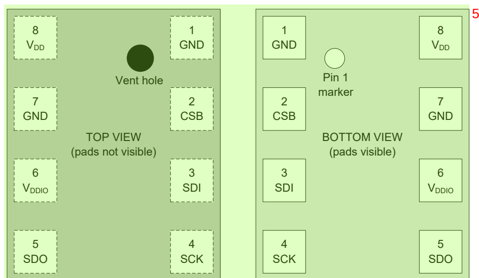
Figure 14: Pin-out top and bottom view 6
