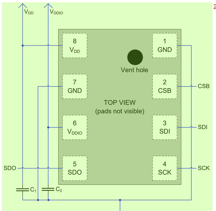
Figure 15: 4-wire SPI connection diagram (Pin1 marking indicated) 3
