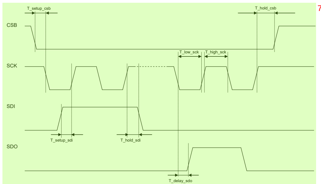
Figure 13: SPI timing diagram 8
