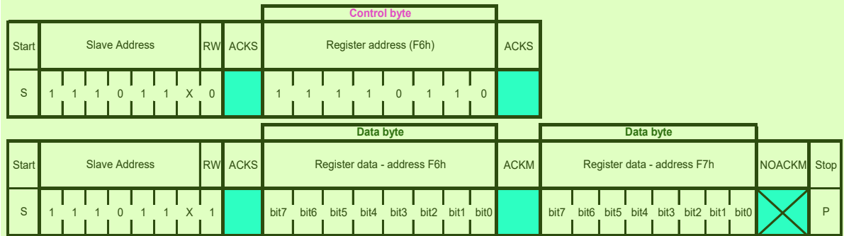
Figure 8: I 2 C multiple byte read 4
