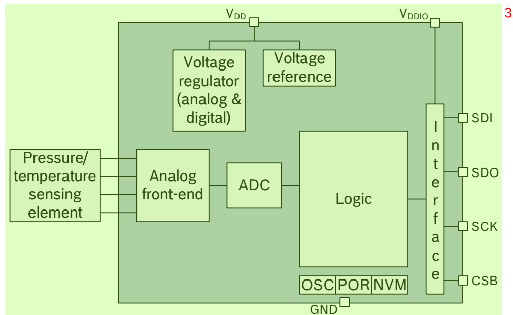
Figure 1: Block diagram of BMP280 4
