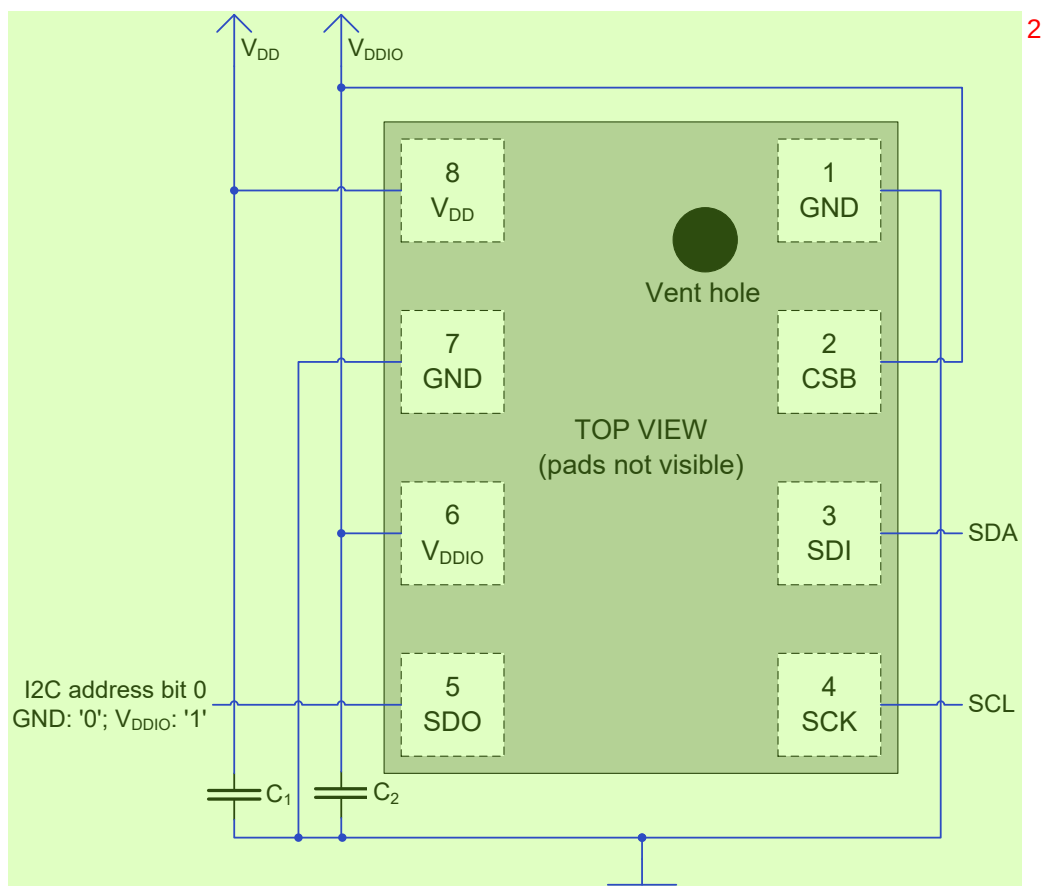
Figure 17: I 2 C connection diagram (Pin1 marking indicated) 3
