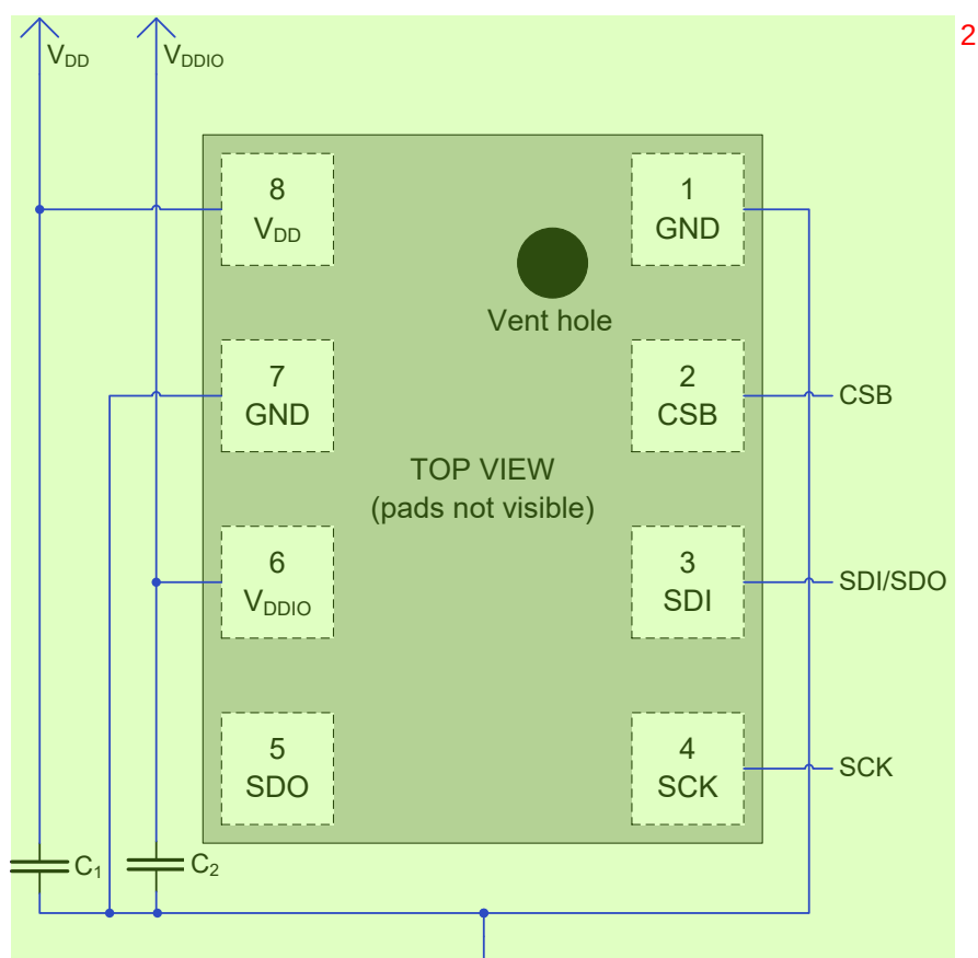
Figure 16: 3-wire SPI connection diagram (Pin1 marking indicated) 3
