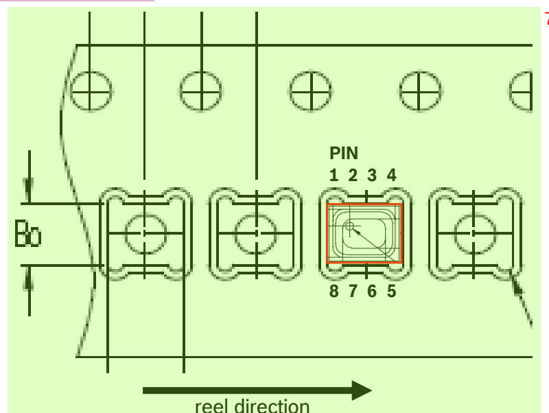
Figure 22: Orientation within tape 8
