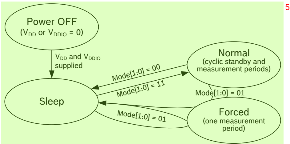
Figure 5: Mode transition diagram 6
