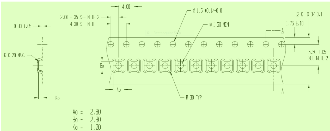
Figure 21: Tape and Reel dimensions 4
