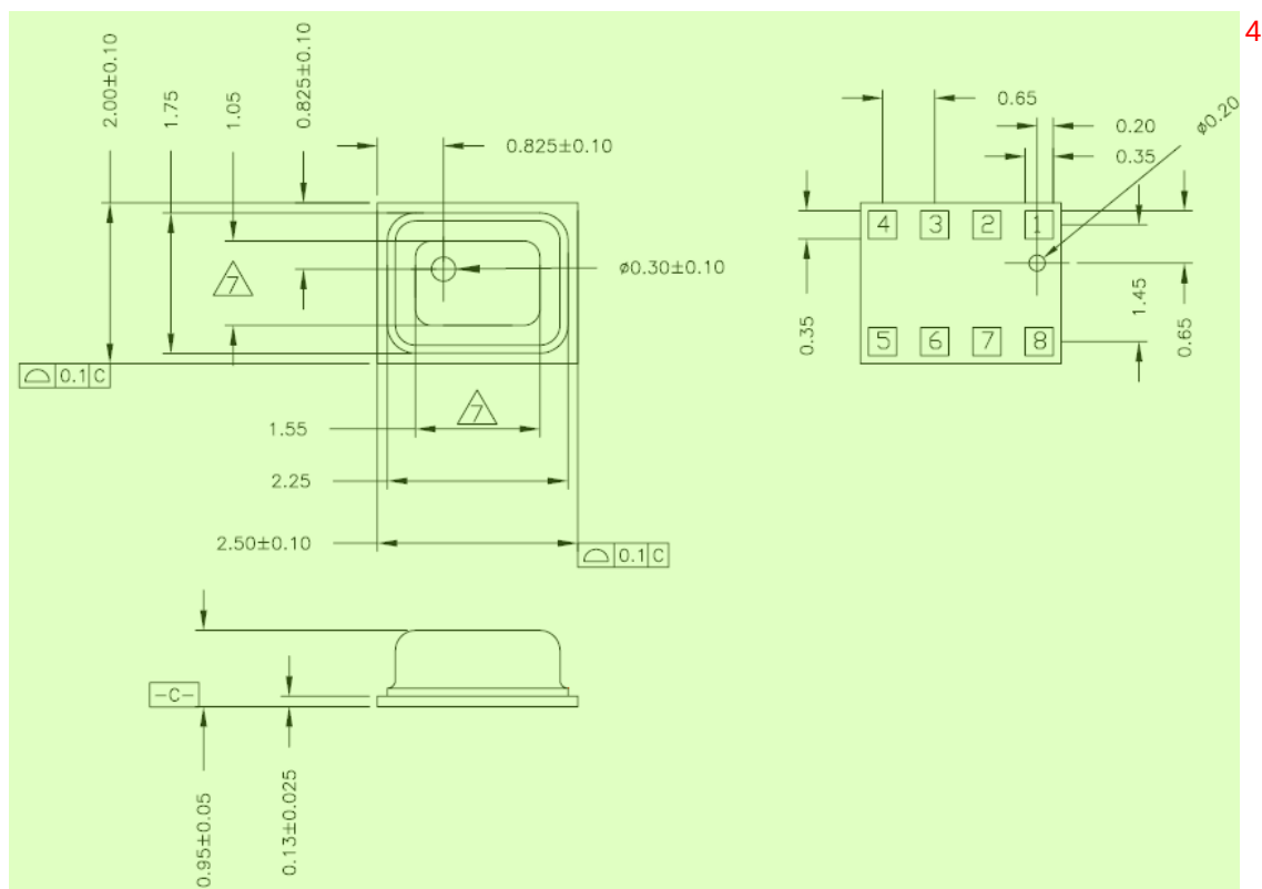
Figure 18: Package outline dimensions for top, bottom and side view 5
