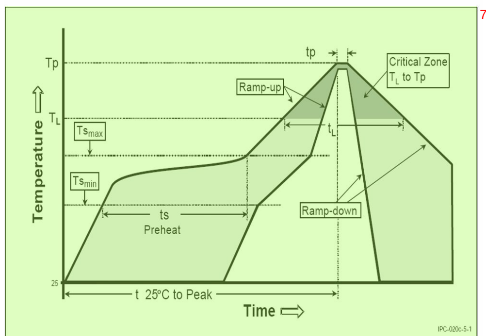
Figure 20: Soldering profile 8
