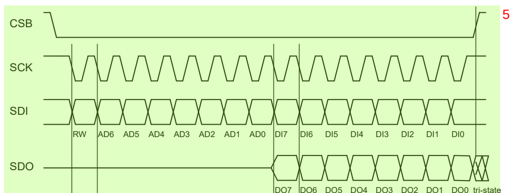
Figure 9: SPI protocol (shown for mode '11' in 4-wire configuration) 6
