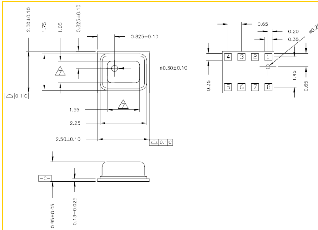
Figure 18: Package outline dimensions for top, bottom and side view
