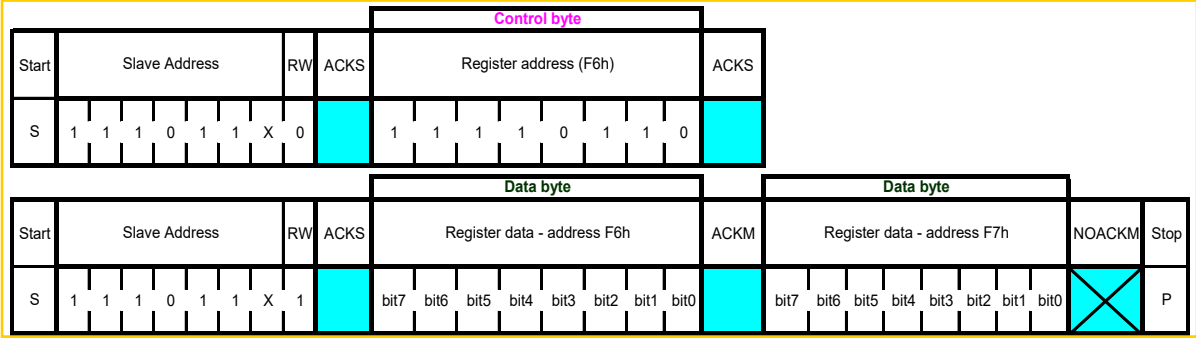
Figure 8: I 2 C multiple byte read
