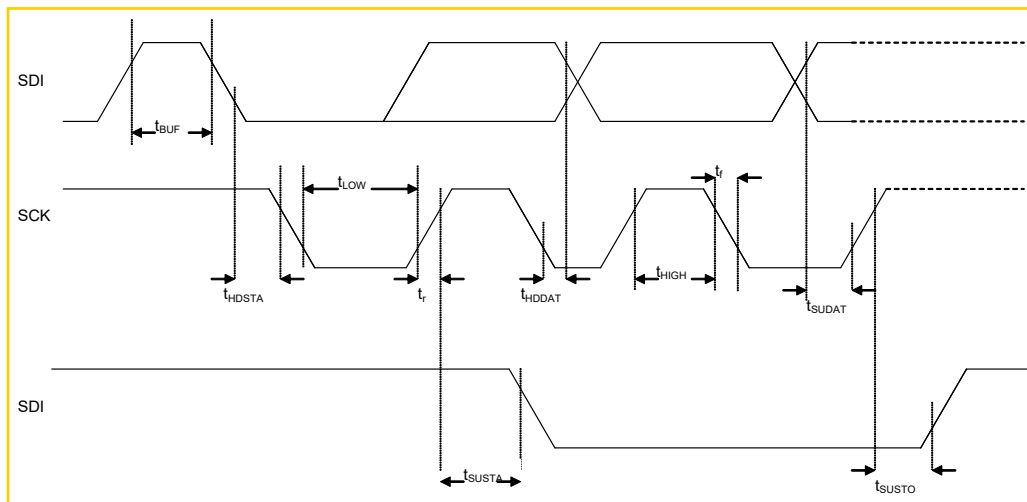
Figure 12: I²C timing diagram
