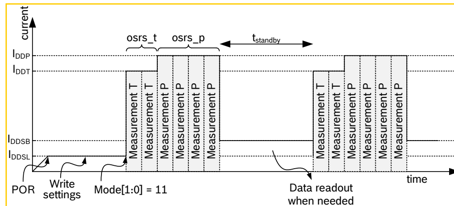
Figure 4: Normal mode timing diagram
