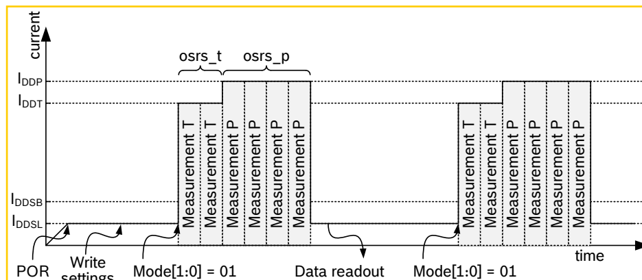
Figure 3: Forced mode timing diagram
