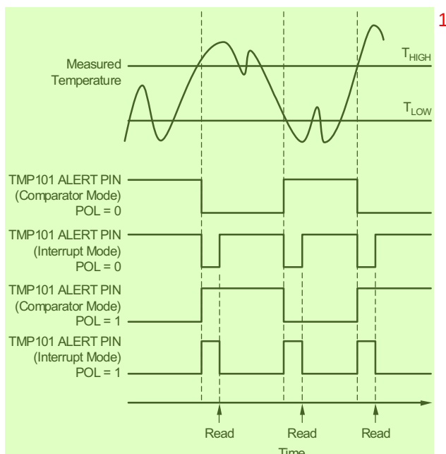
Figure 11. Output Transfer Function Diagrams 2
