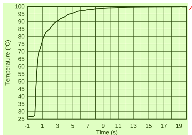
Figure 14. Temperature Step Response 5
