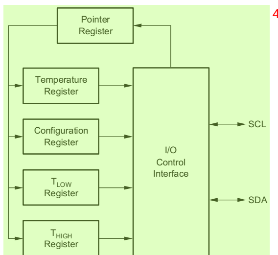
Figure 10. Internal Register Structure of the TMP100 and TMP101 5
