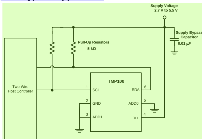
Figure 12. Typical Connections of the TMP100 9
