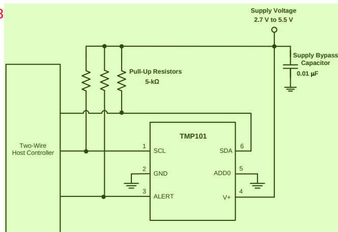
Figure 13. Typical Connections of the TMP101 11
