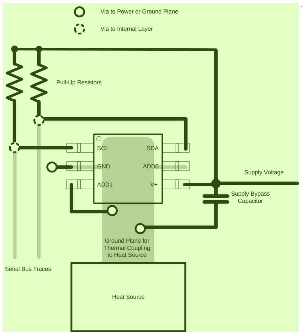
Figure 15. TMP100 Layout Example 8
