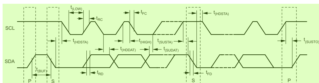
Figure 6. I 2 C Timing Diagram 11
