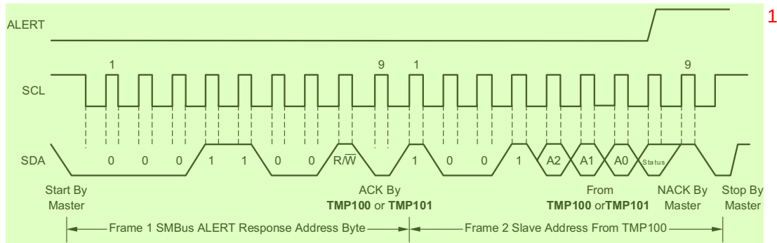
Figure 9. Timing Diagram for SMBus ALERT
