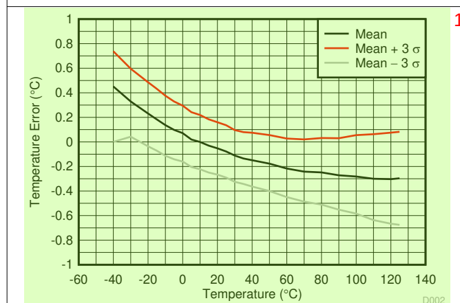
Figure 5-5. Temperature Error vs Temperature 12
