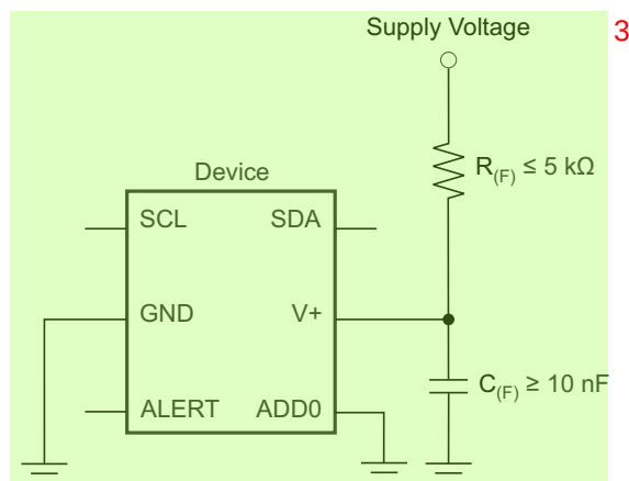
Figure 7-2. Noise Reduction Techniques
