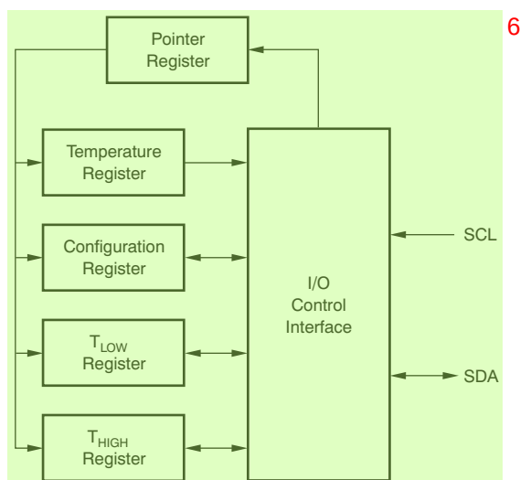
Figure 6-6. Internal Register Structure 6
