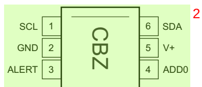
Figure 4-1. DRL Package 6-Pin SOT563 Top View 3
