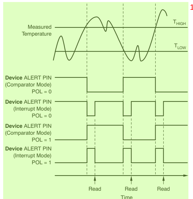
Figure 6-7. Output Transfer Function Diagrams 2
