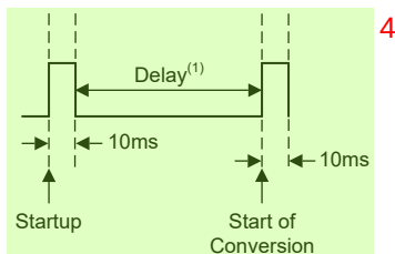
Figure 6-5. Conversion Start
