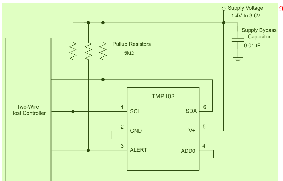
Figure 7-1. Typical Connections
