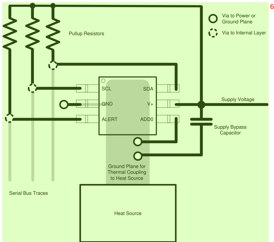
Figure 7-4. TMP102 Layout Example
