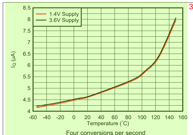
Figure 5-1. Average Quiescent Current vs Temperature 4
