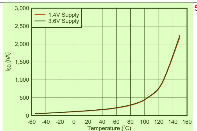
Figure 5-2. Shutdown Current vs Temperature 6
