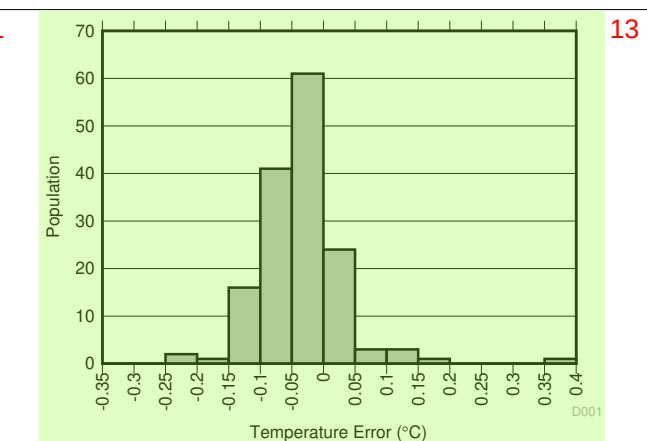
Figure 5-6. Temperature Error at 25°C 14
