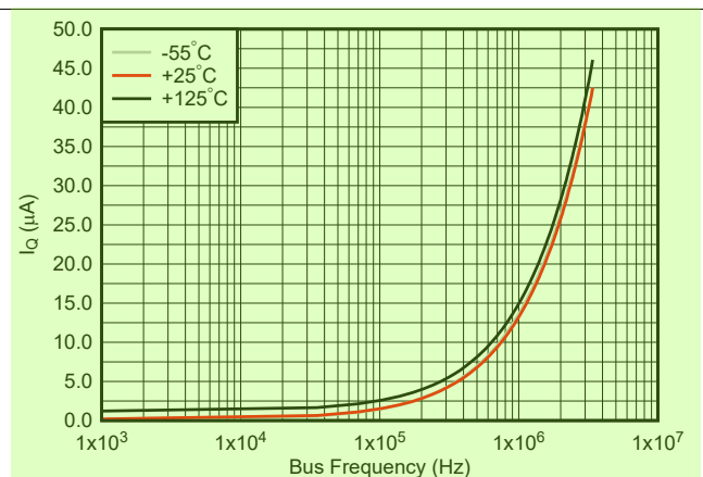
Figure 5-4. Quiescent Current vs Bus Frequency (Temperature at 3.3-V Supply) 10
