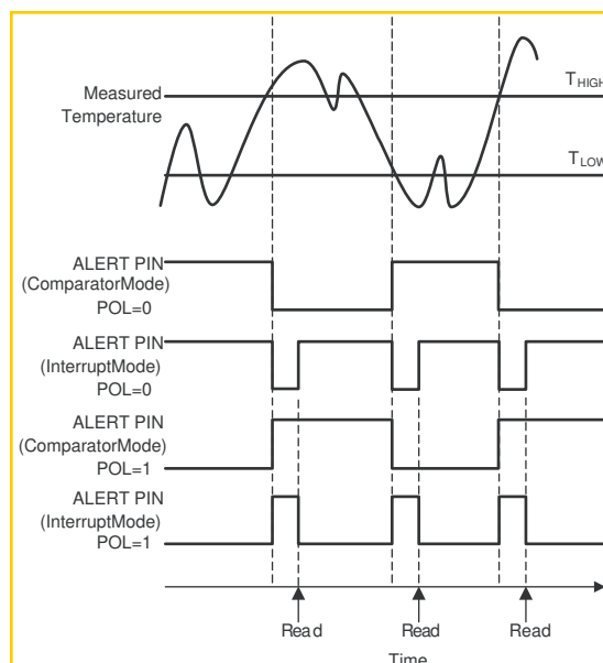
Figure 7-10. Output Transfer Function Diagrams
