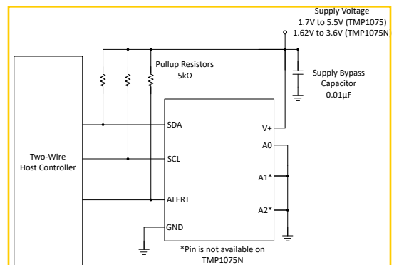
Simplified Schematic
