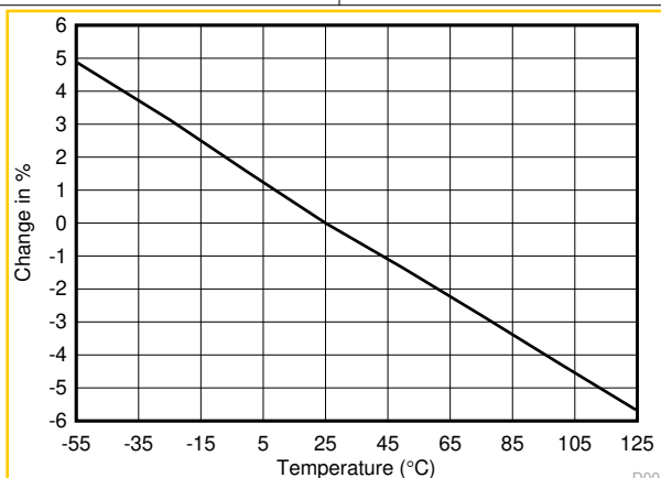
Figure 6-10. Sampling Period Change vs. Temperature (1.7 V to 5.5 V)
