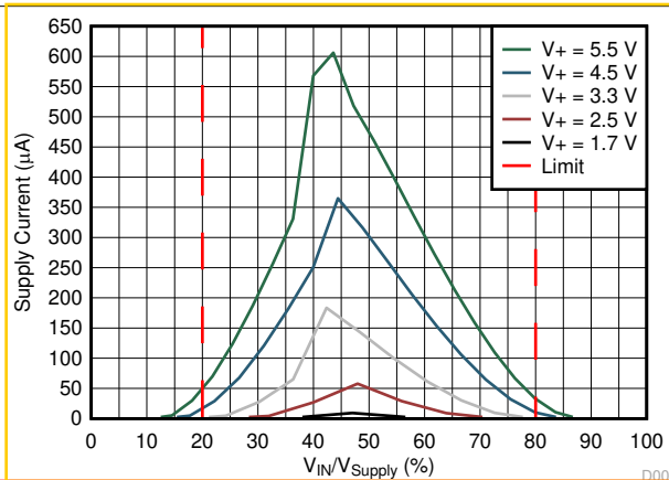
Figure 6-7. Supply Current vs. Input Cell Voltage
