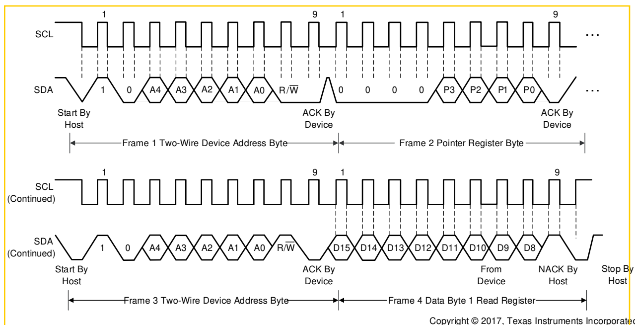
Figure 7-6. Two-Wire Timing Diagram for Read Single Byte Format
