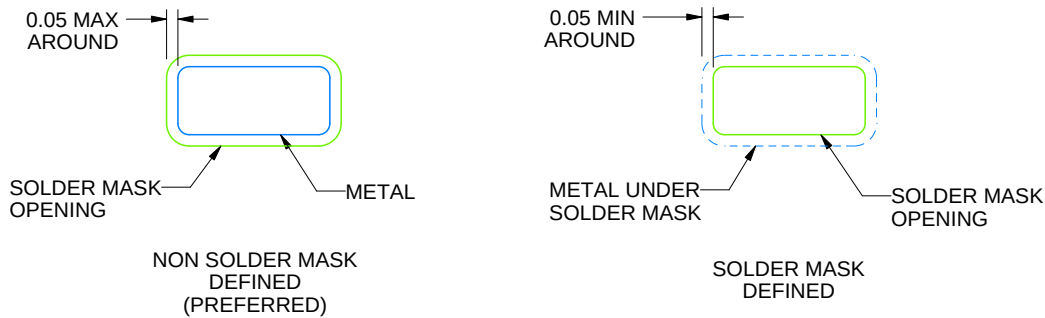
SOLDERMASK DETAILS
