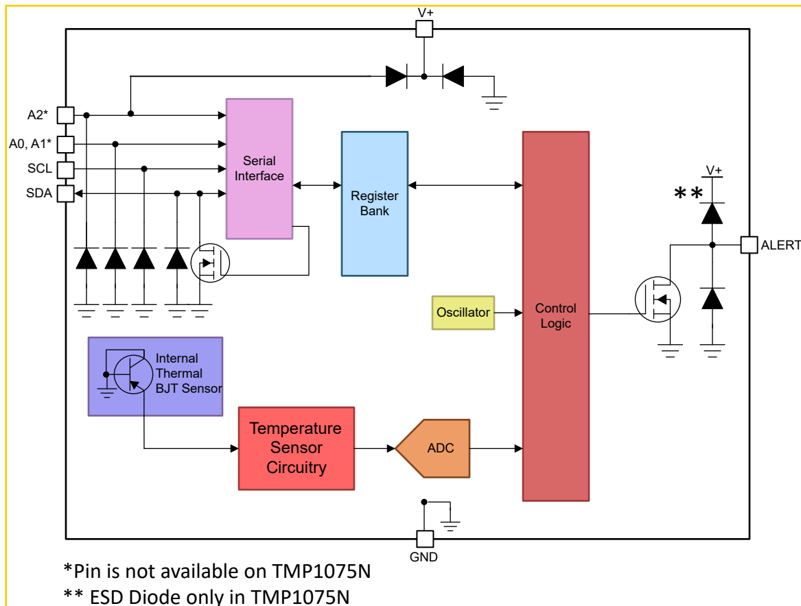
Figure 7-1. Functional Block Diagram
