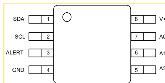
Figure 5-2. DGK Package 8-Pin VSSOP Top View
