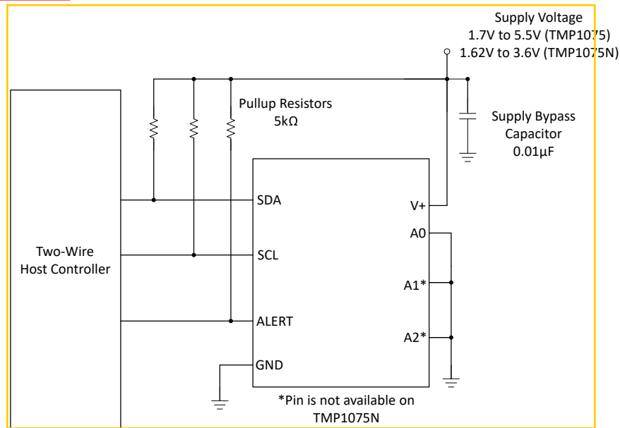
Figure 8-1. Typical Connections
