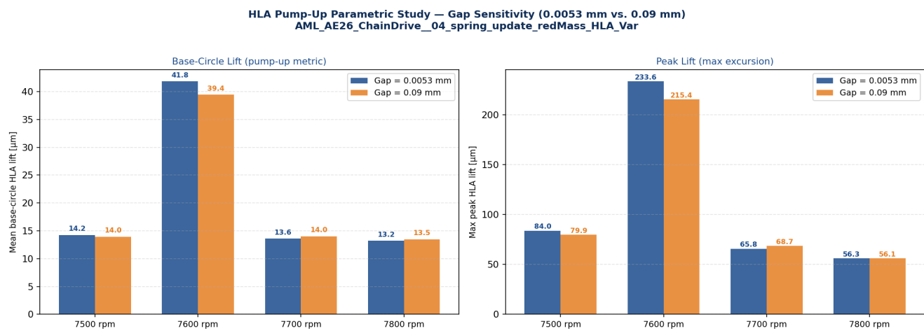
Fig. 10-1: Gap Sensitivity - Base-Circle Lift and Peak Lift by Speed. Left: mean base-circle HLA lift (pump-up metric) for tight-gap (blue) and loose-gap (orange) cases at 7500-7800 rpm. Right: maximum peak lift per case. The 7600 rpm point is elevated in both gap cases due to valvetrain resonance; the gap delta is only 2.4 \mu m (6%).
