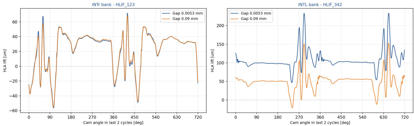
Fig. 10-2: HLA Lift Waveform at 7600 rpm - Tight vs. Loose Gap (Last 2 Cycles). HLIF_123 (INTr right bank) and HLIF_342 (INTL left bank). Both gap sizes produce large dynamic excursions at 7600 rpm resonance. The loose gap shows higher peak-to-peak amplitude (215 um vs 149 um) due to lower mean offset.
