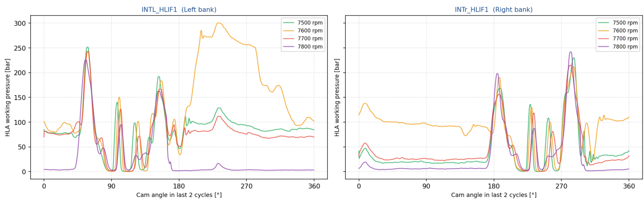
Fig. 4-4: HLA Working Pressure — Last 2 Cam Cycles Working pressure in the HLA oil column over the last two cycles. An elevated or oscillating working pressure in the base-circle phase (between lift events) corroborates pump-up detected via the lift signal.
