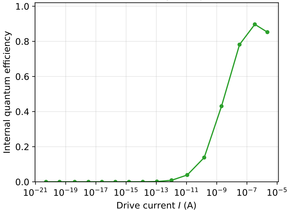
DH LED efficiency vs injection
