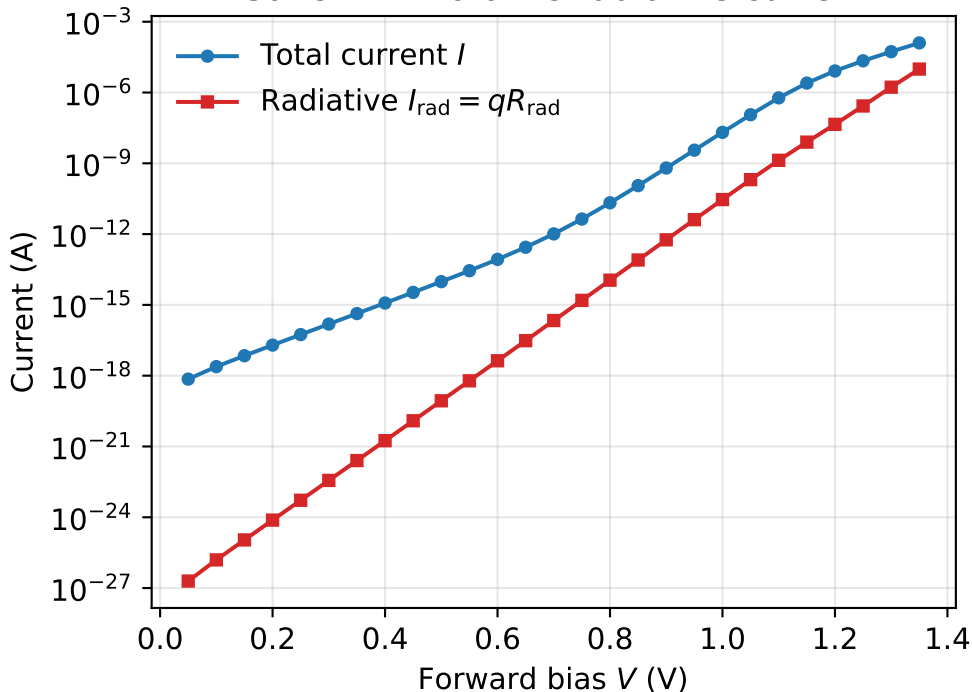
GaAs LED: total vs radiative current
