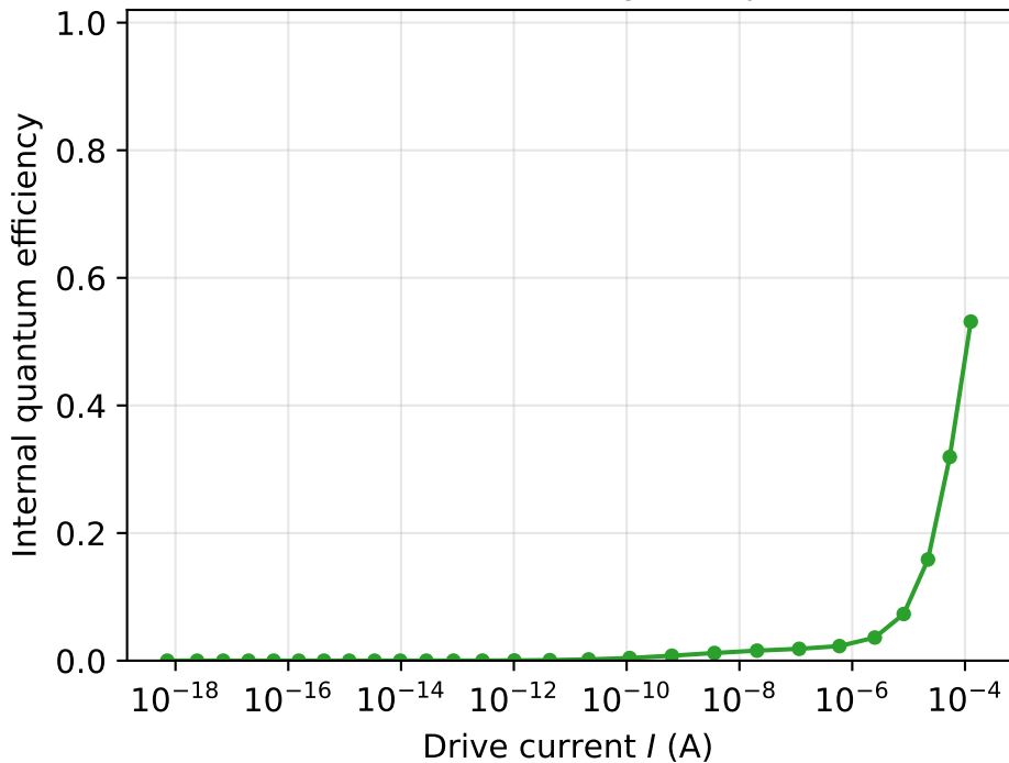
GaAs LED efficiency vs injection
