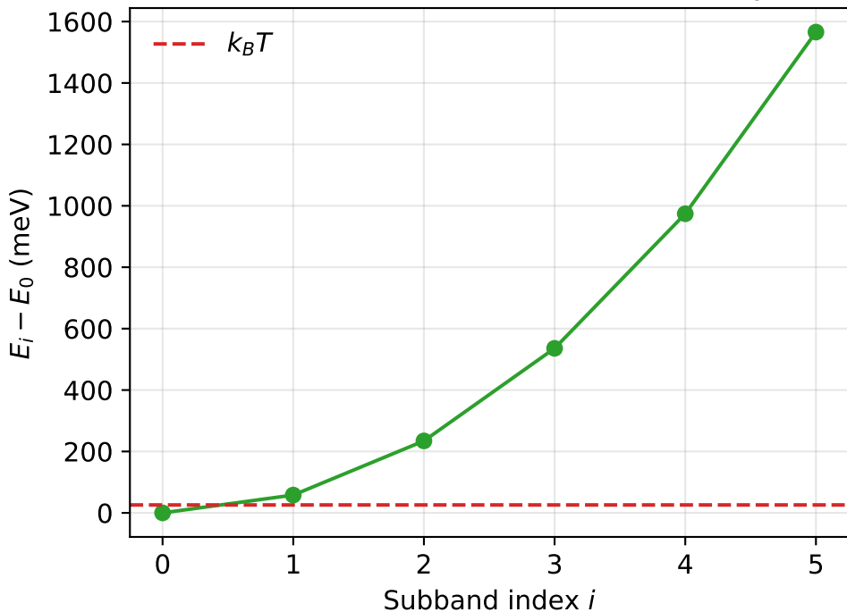
Electron subband ladder (5 nm body)
