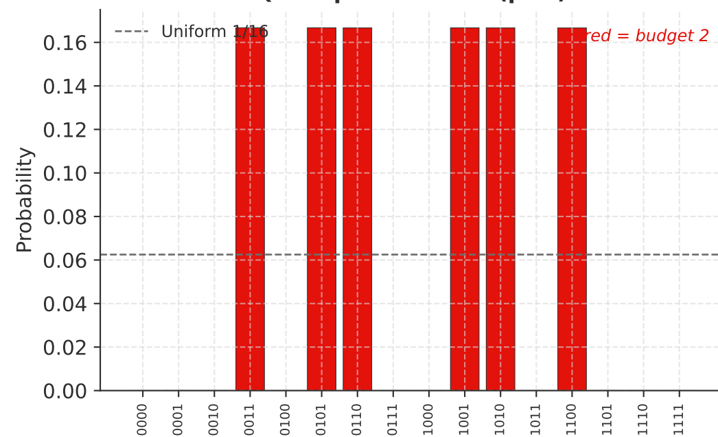
QAOA probabilities (p=2)
