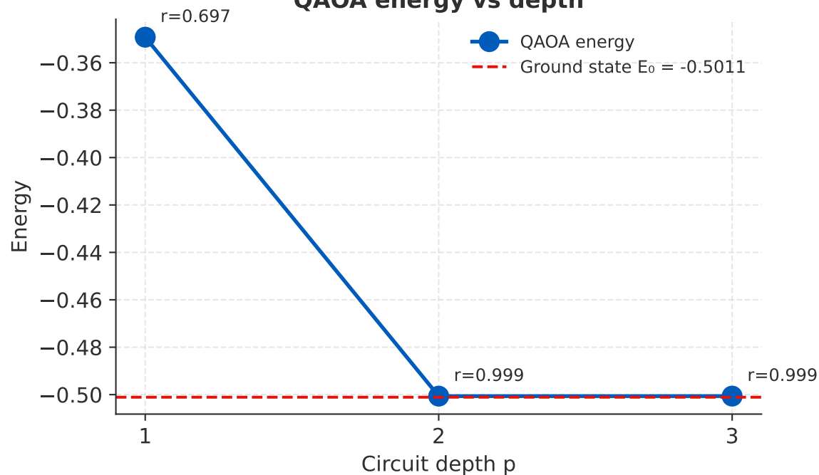
QAOA energy vs depth
