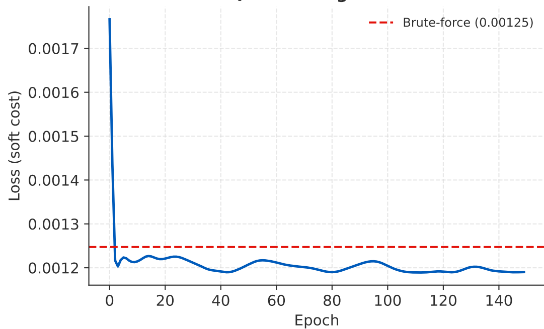
QNN training curve
