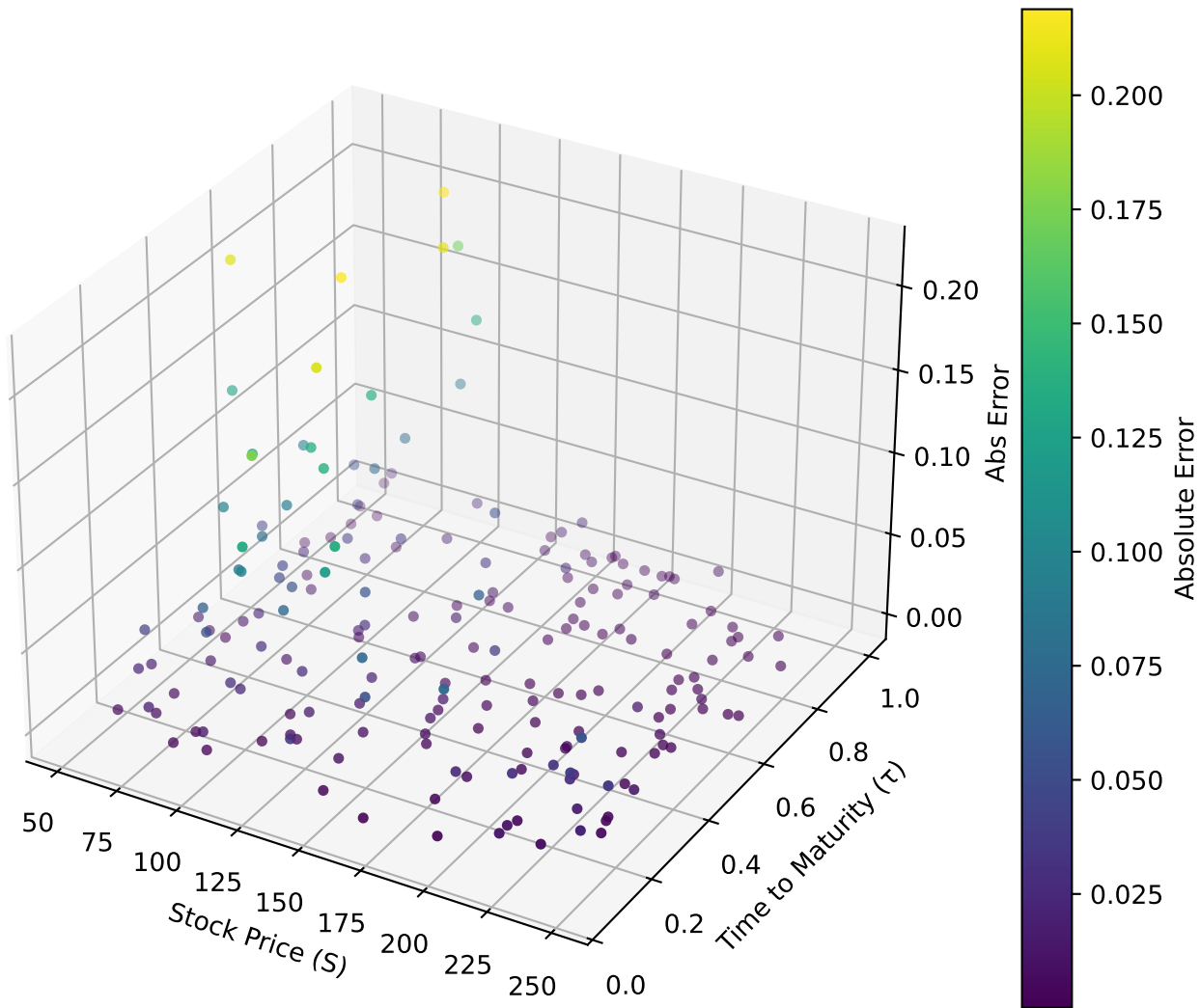
Inverse PINN: Prediction Error Across Data Points
