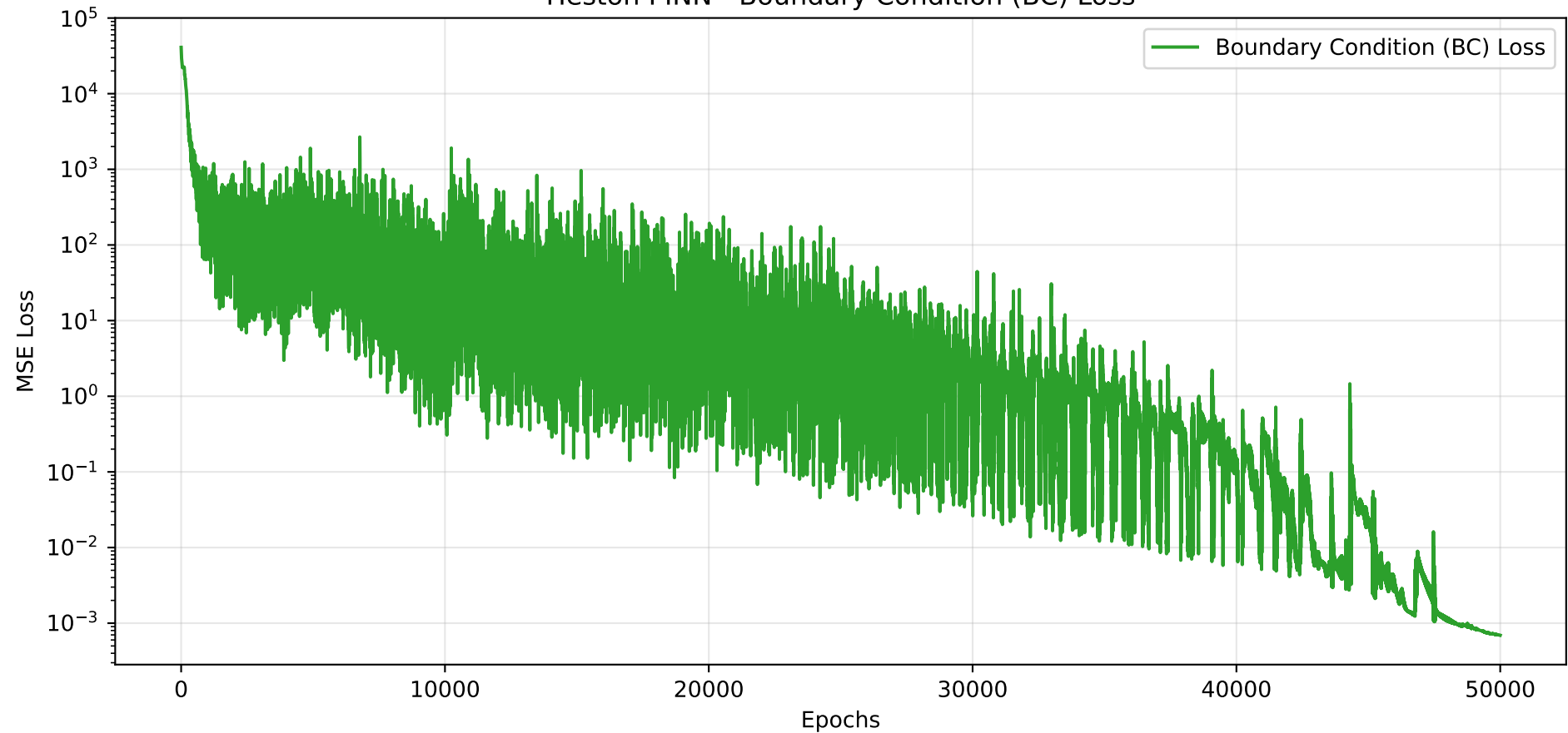
Heston PINN - Boundary Condition (BC) Loss
