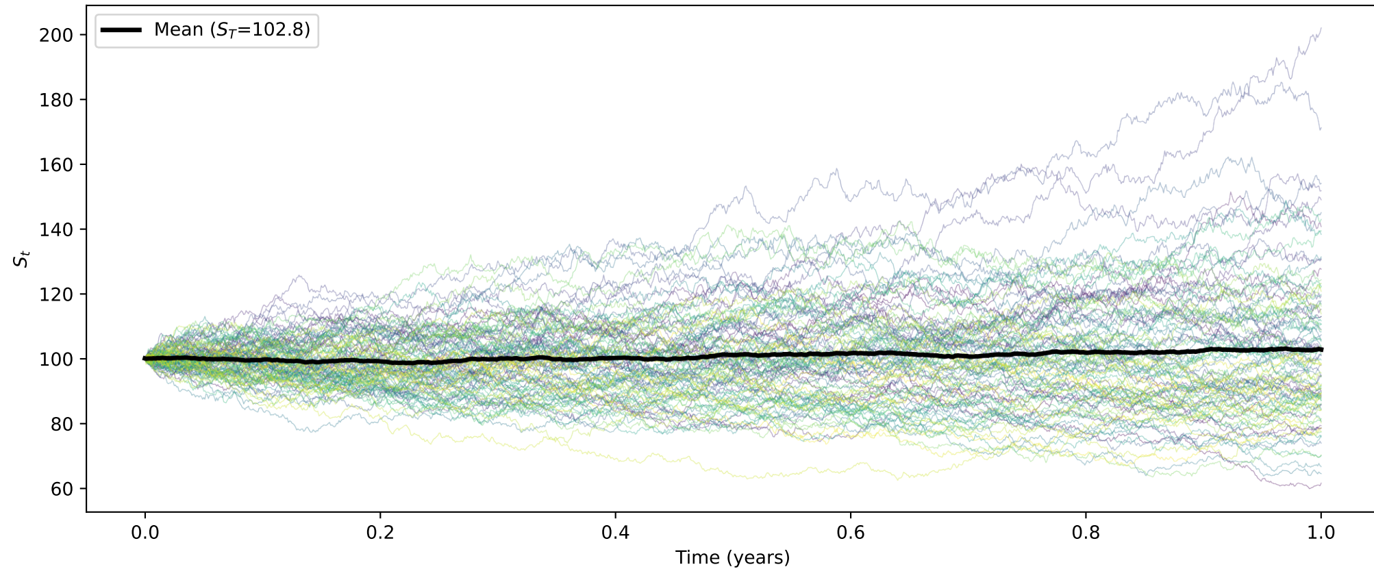
Geometric Brownian Motion (100 paths, S_0=100.0 , \mu=0.05 , \sigma=0.2 )
