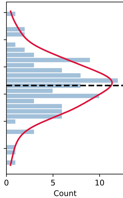
S_T dist.
