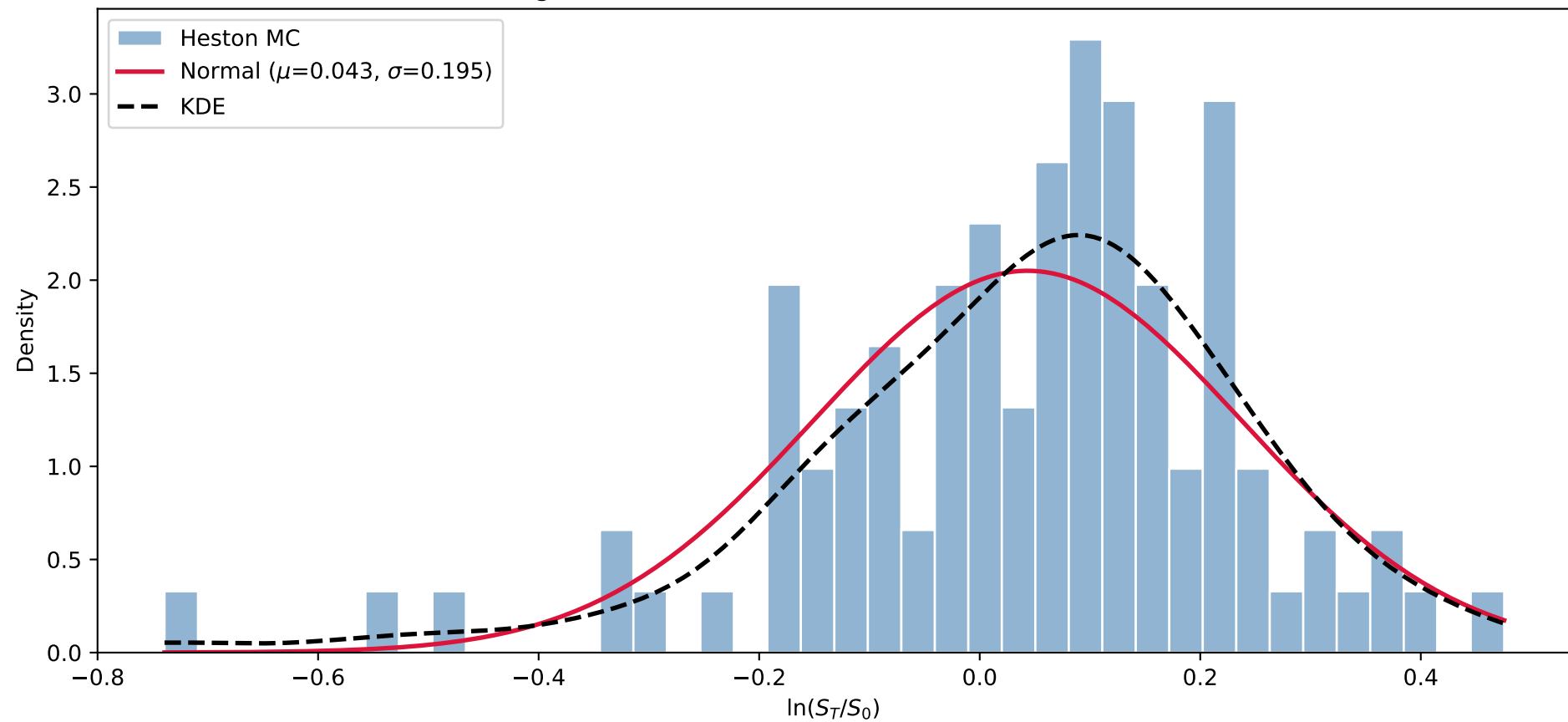
Terminal Log-Return Distribution (skew=-0.966, excess kurt=2.271)
