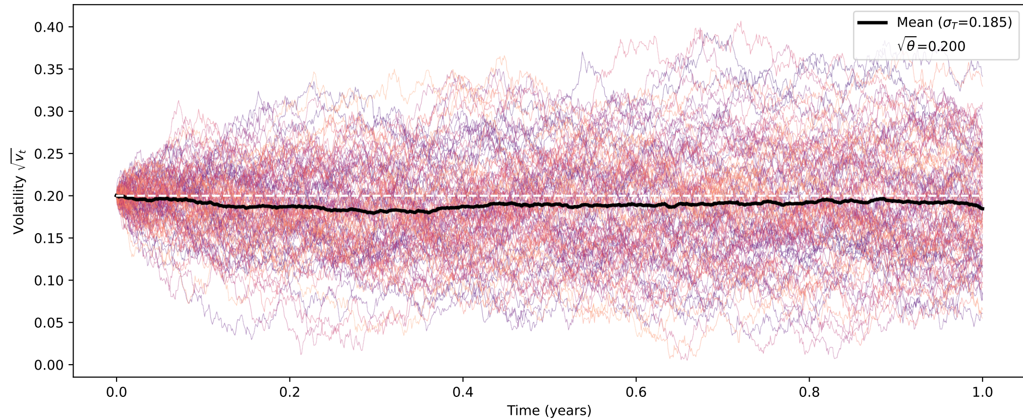
Stochastic Volatility \sqrt{v_t} ( \kappa=2.0 , \theta=0.04 , \xi=0.3 )
