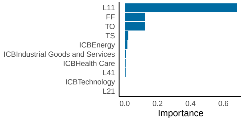
Variable Importance Plot XGBB30
