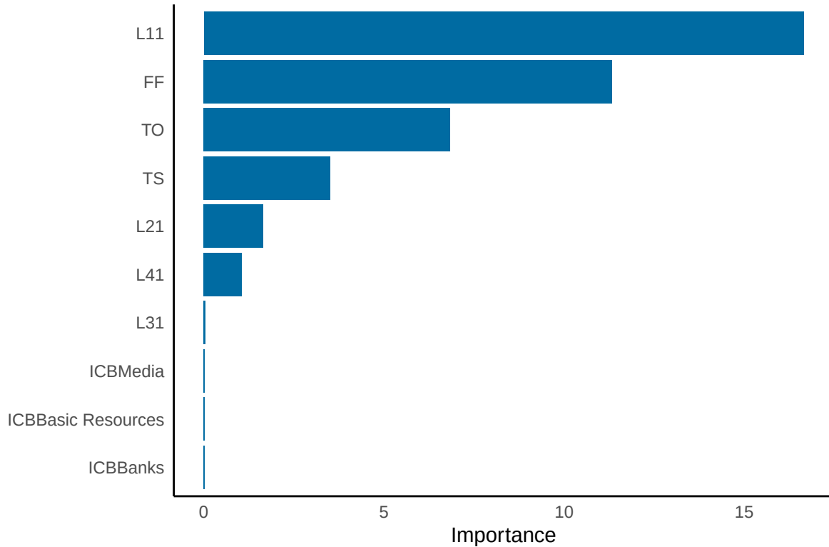
Variable Importance Plot GLM30
