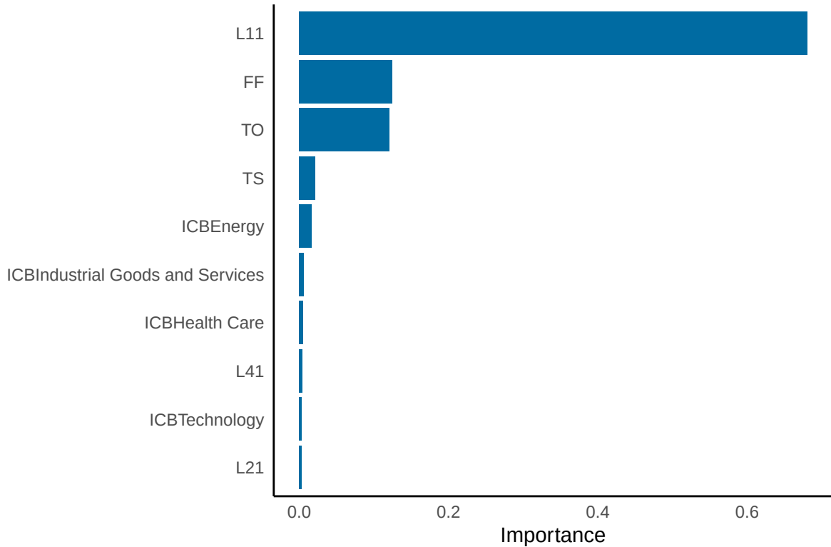
Variable Importance Plot XGBB30
