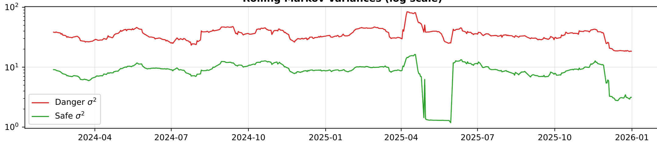
Rolling Markov Variances (log scale)
