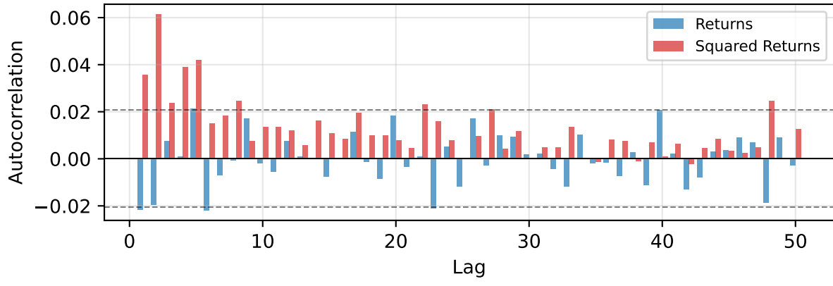
ACF of GBPUSD: Returns vs r 2 (50 lags)
