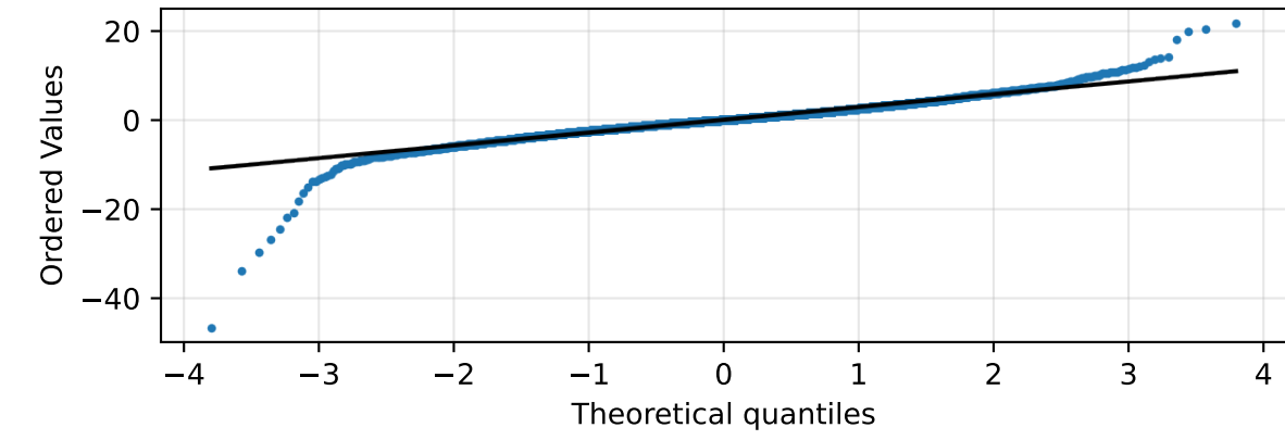
Q-Q Plot vs Normal (GBPUSD)
