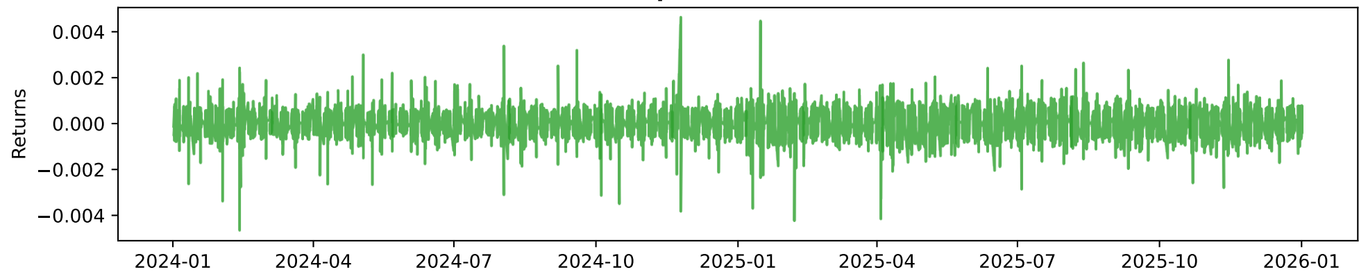
Spread Returns
