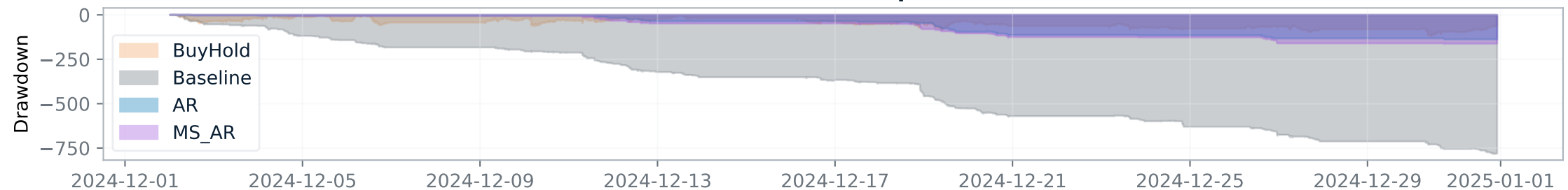
Drawdown (bps)
