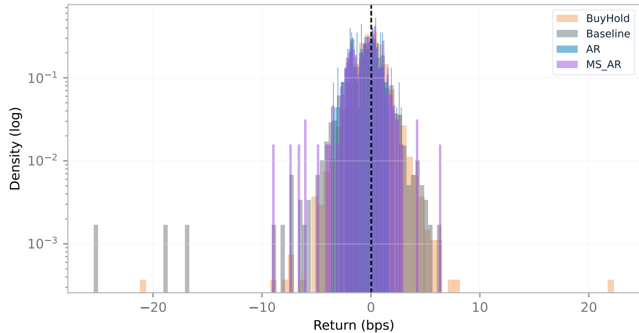
Return distribution (log y, tails visible)
