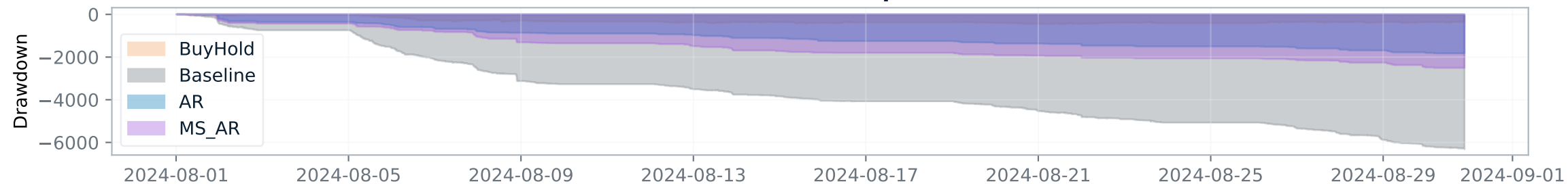
Drawdown (bps)
