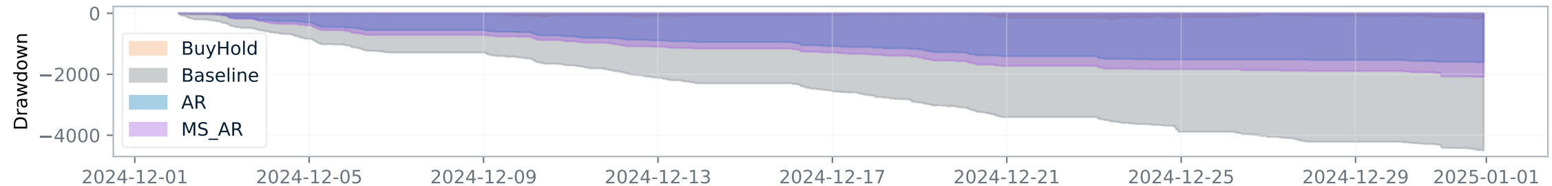
Drawdown (bps)
