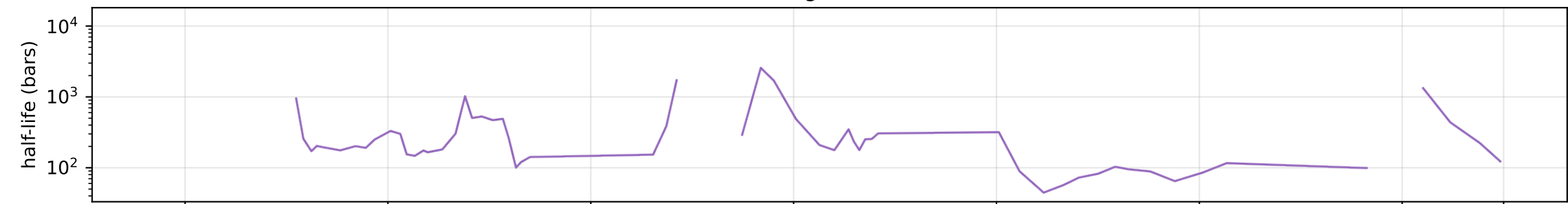
Rolling Half-Life
