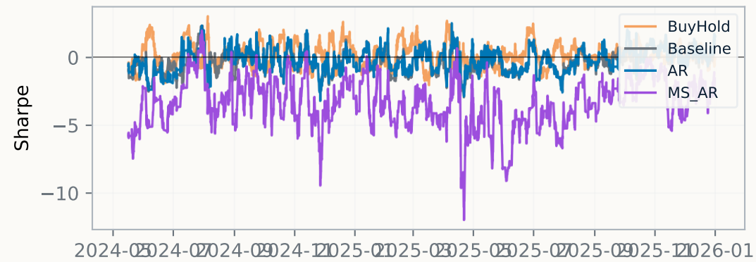
Rolling Sharpe (642-bar window)
