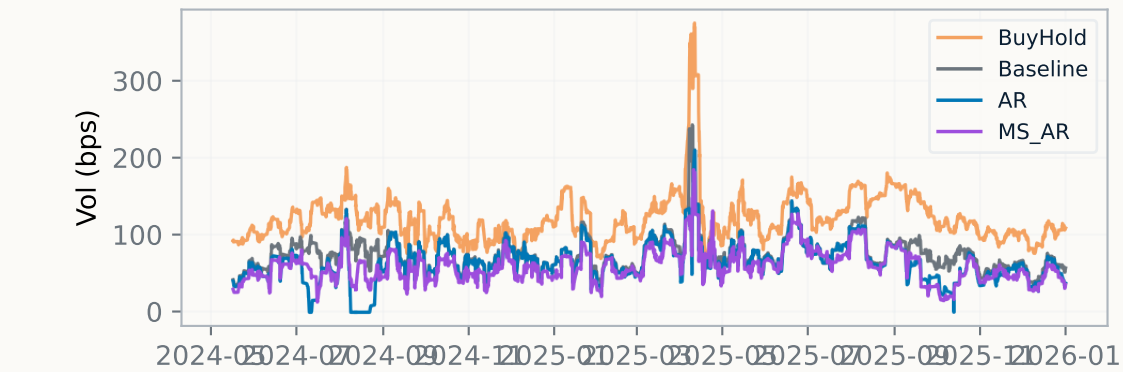
Rolling Volatility (642-bar window)
