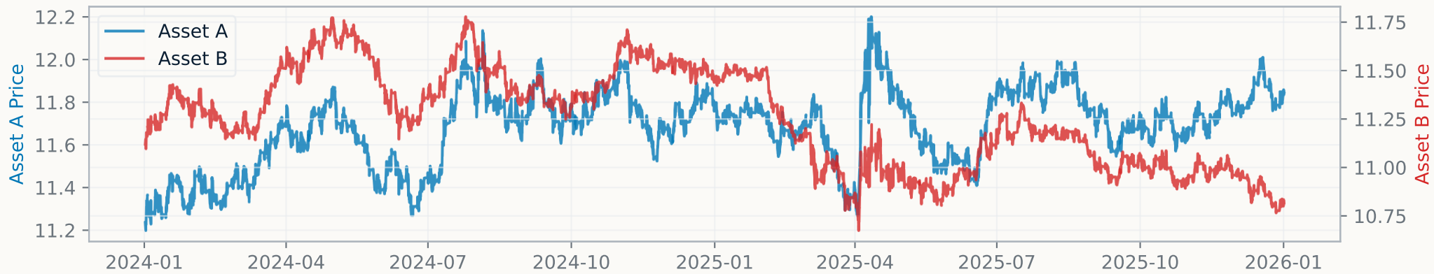
Asset Prices (Time Series)
