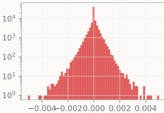
Return B Dist (Log Scale)
