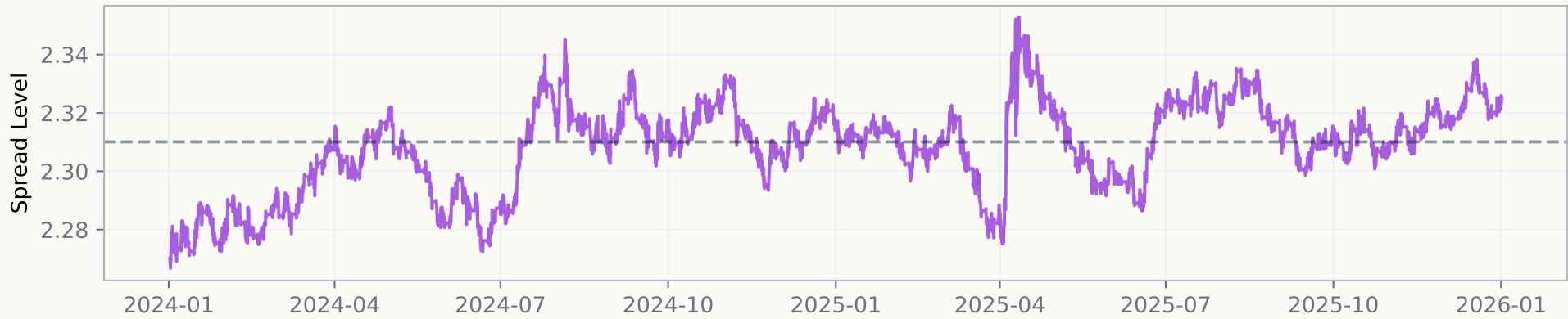
Log Spread (Log A - 0.062 * Log B)
