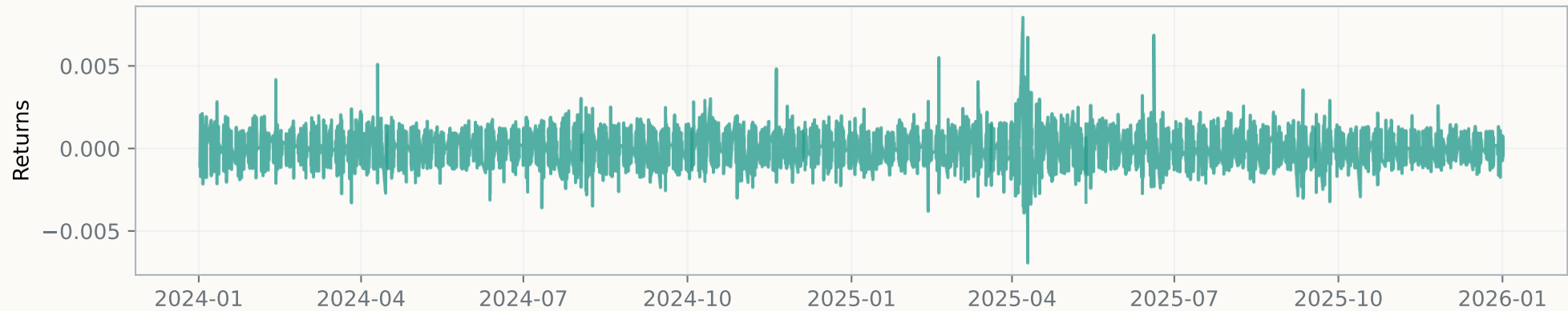
Spread Returns
