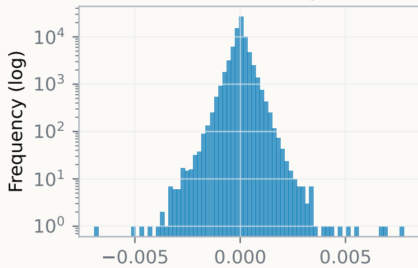
Return A Dist (Log Scale)
