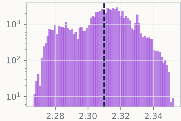
Spread Level Dist (Log Scale)
