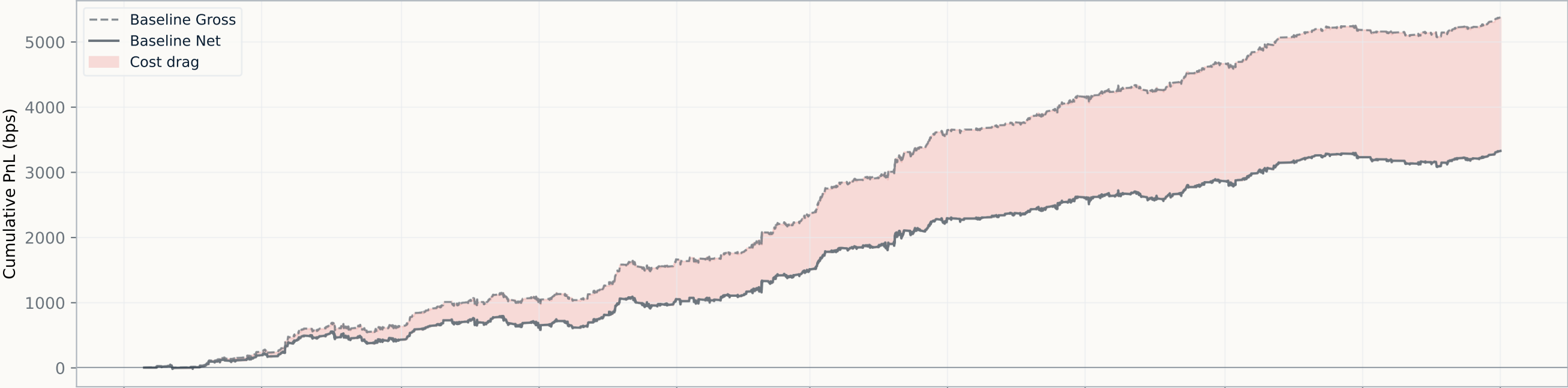
AR: Gross vs Net Returns
