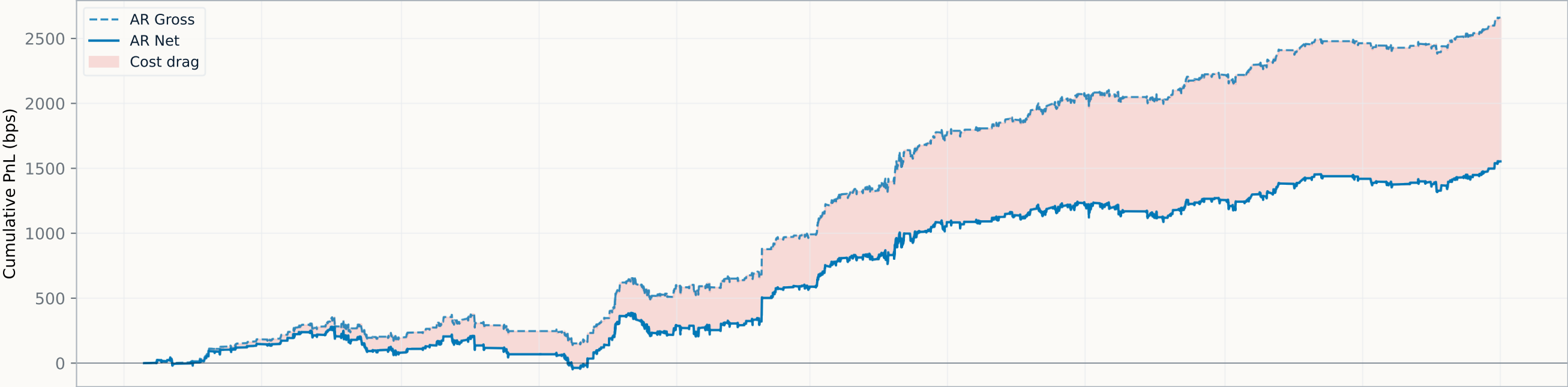
MS_AR: Gross vs Net Returns
