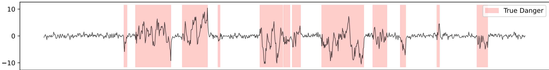
Time Series with True Hidden States
