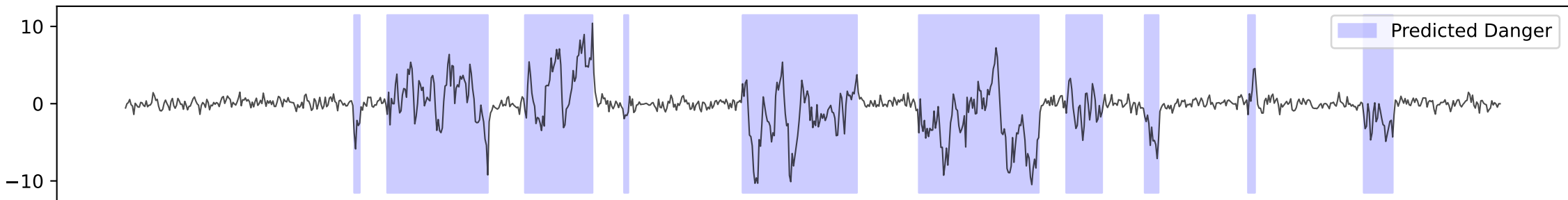
MS-AR Identified Regimes
