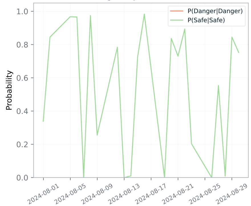
Regime persistence
