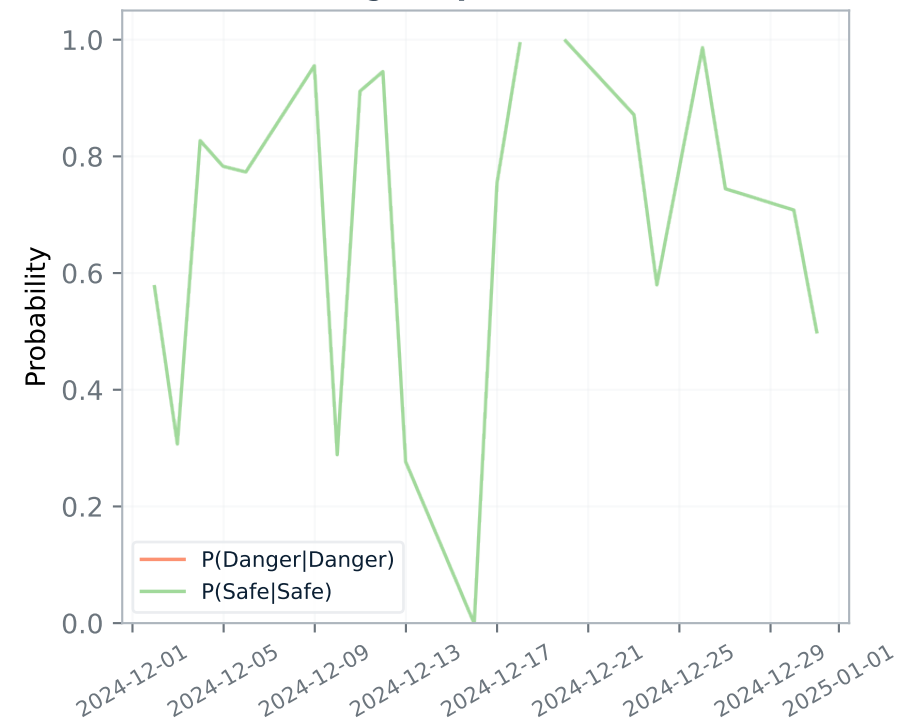
Regime persistence
