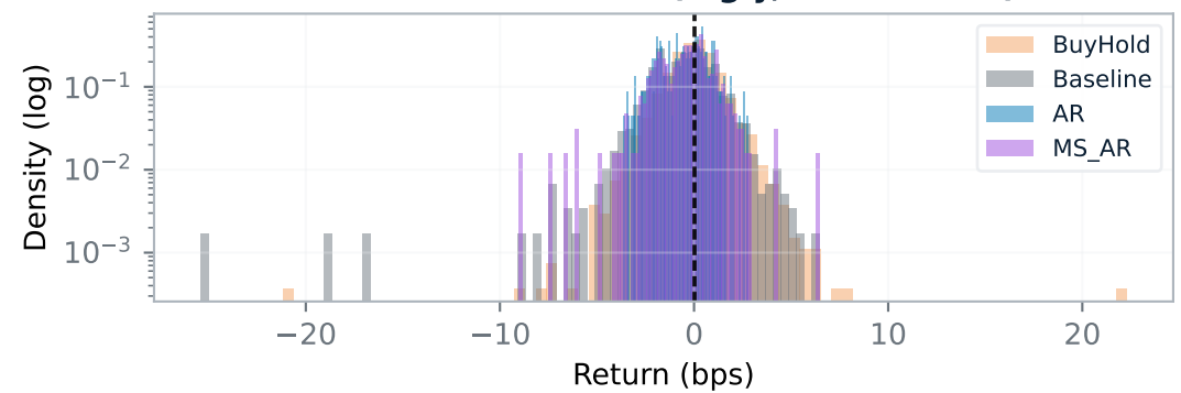
Return distribution (log y, tails visible)
