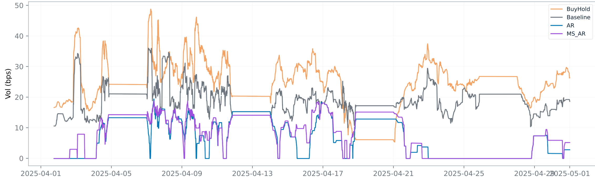
Rolling volatility (200-bar window)
