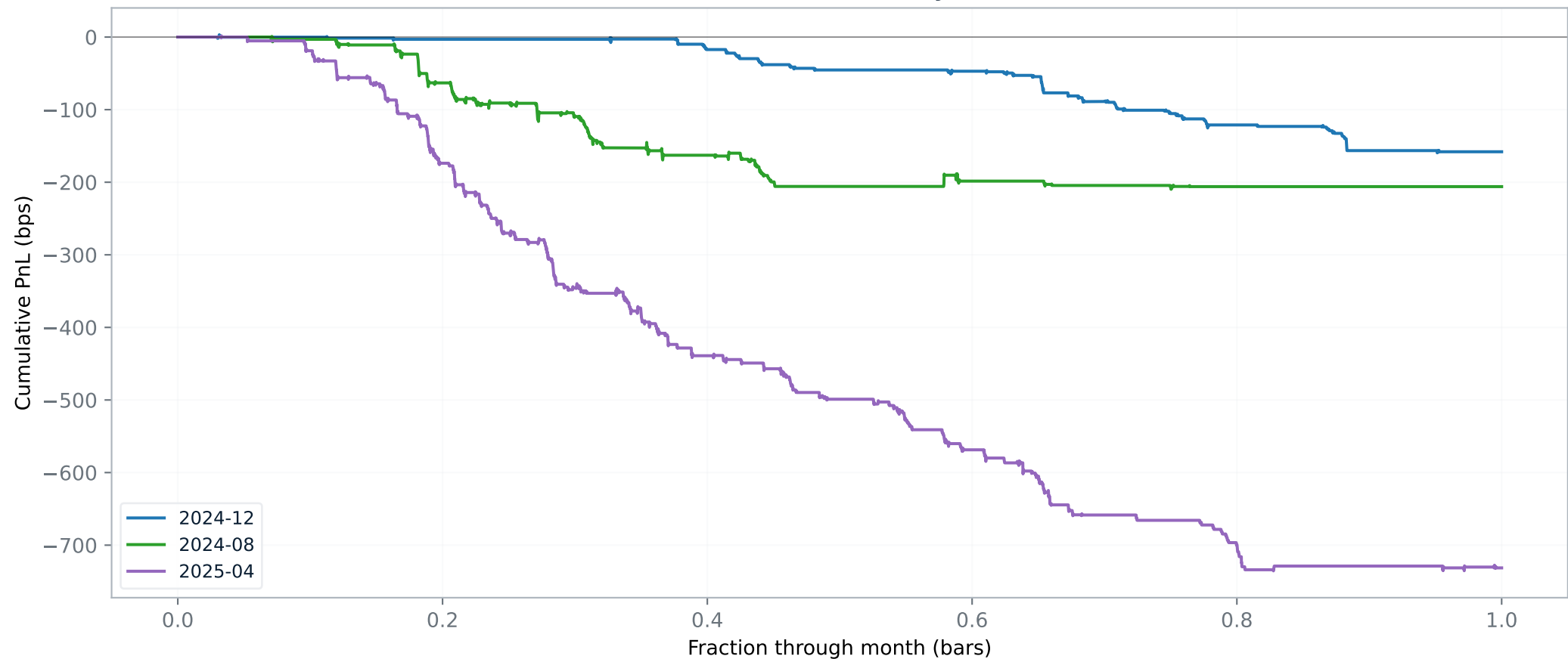
AUDUSD/NZDUSD — (4) MS-AR (dynamic threshold)
