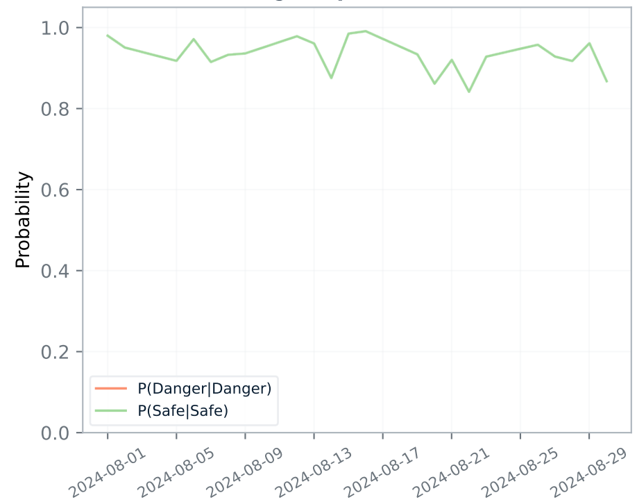
Regime persistence
