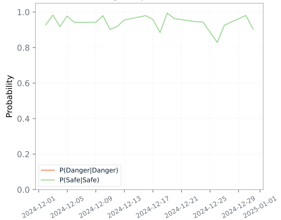
Regime persistence
