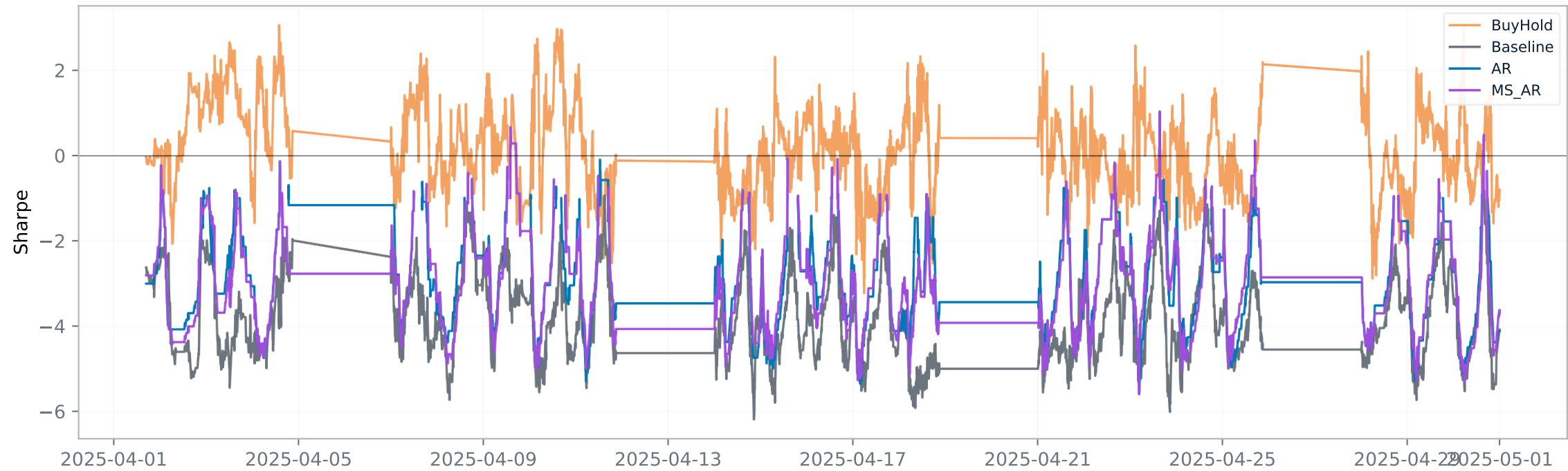
Rolling Sharpe (261-bar window)
