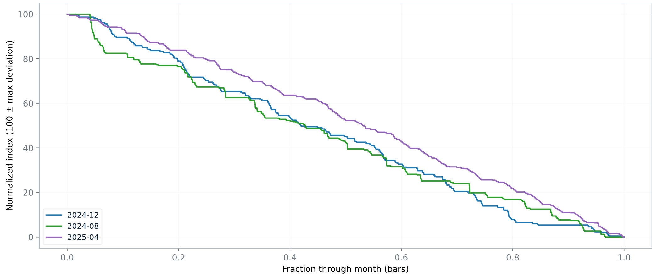
EURNOK/EURSEK — (3) AR (binary gate) — normalized \pm 100
