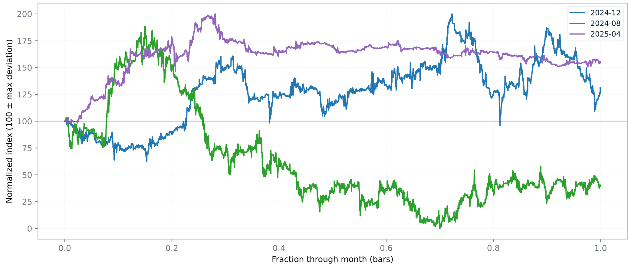
EURNOK/EURSEK — (1) Buy & Hold — normalized \pm 100
